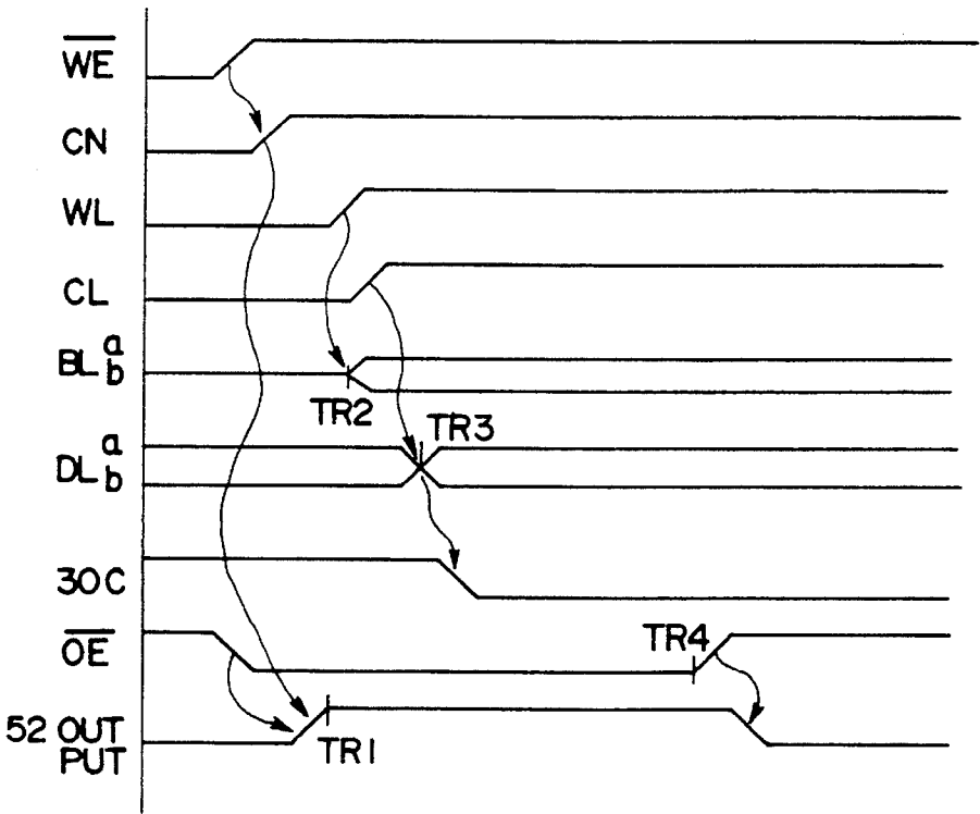
FIG. 2 READ OPERATION
