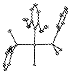
\text{PMe}_2\text{Ph} (109)
