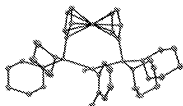
dcpf (117)
