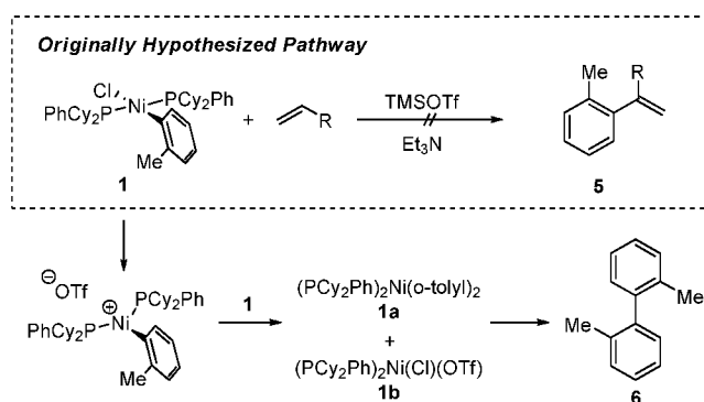
Scheme 3. Activation of Precatalyst 1
