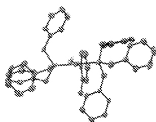
\text{PBn}_3 (106)
