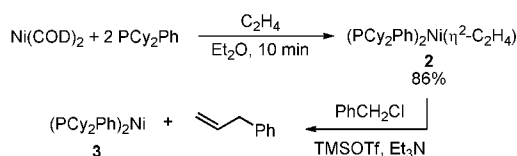
Scheme 1. Synthesis of (PCy 2 Ph) 2 Ni(η 2 -C 2 H 4 )
