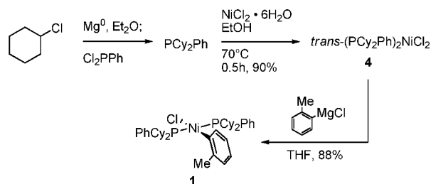
Scheme 2. Synthesis of trans-(PCy 2 Ph) 2 Ni(o-tolyl)Cl
