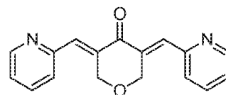
SYC-957 (Compound 4-9)
