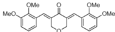
SYC-953 (Compound 4-3)
