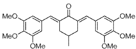
SYC-949 (Compound 3-5)
