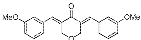
SYC-850 (Compound 4-2)
