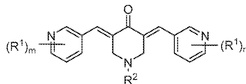
Structure I-A3
