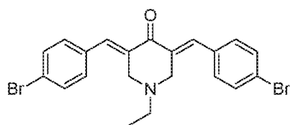
SYC-966 (Compound 6-7)
