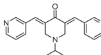
SYC-855 (Compound 7-8)
