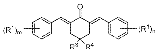
Structure I-B1
