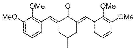
SYC-947 (Compound 3-3)
