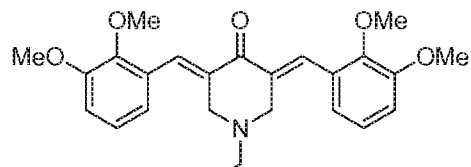
SYC-963 (Compound 6-3)
