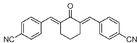
Compound S18
