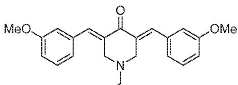
SYC-962 (Compound 6-2)
