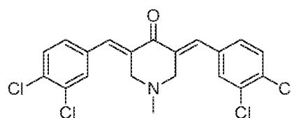
SYC-959 (Compound 5-6)
