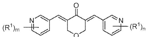
Structure I-C2
