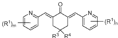
Structure I-B2
