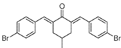
SYC-951 (Compound 3-7)
