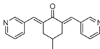
SYC-909 (Compound 3-8)
