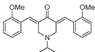
SYC-967 (Compound 7-1)
