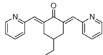
SYC-908 (Compound 2-9)
