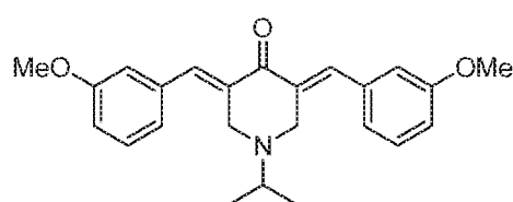
SYC-968 (Compound 7-2)
