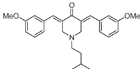
Compound 10-2
