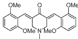
SYC-853 (Compound 5-4)
