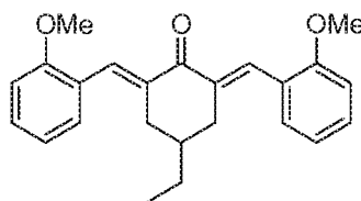
SYC-937 (Compound 2-1)
