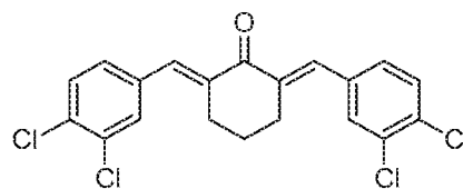
SYC-934 (Compound 1-6)
