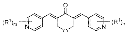
Structure I-C4
