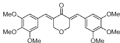
SYC-910 (Compound 4-5)
