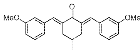
SYC-946 (Compound 3-2)
