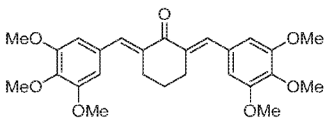
SYC-933 (Compound 1-5)
