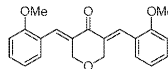
SYC-909 (Compound 3-8)
