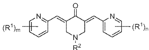
Structure I-A2
