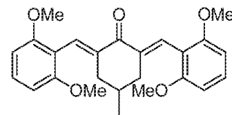
SYC-948 (Compound 3-4)
