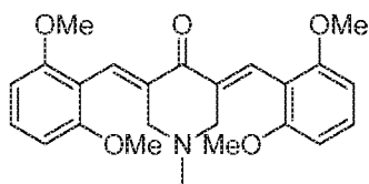
SYC-962 (Compound 6-2)
