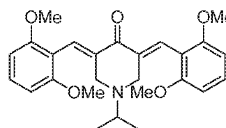
SYC-969 (Compound 7-4)
