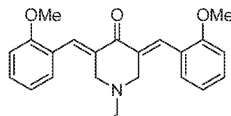
SYC-961 (Compound 6-1)
