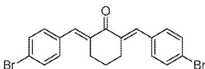
SYC-935 (Compound 1-7)
