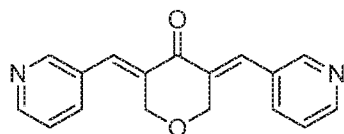
SYC-851 (Compound 4-8)
