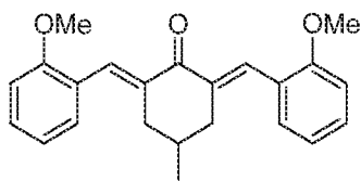
SYC-945 (Compound 3-1)
