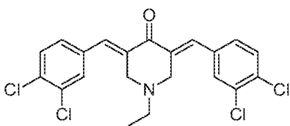
SYC-965 (Compound 6-6)
