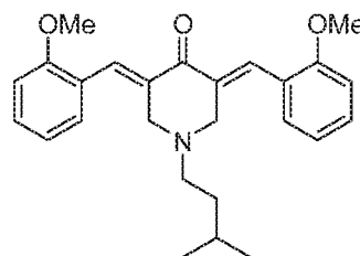
Compound 10-1
