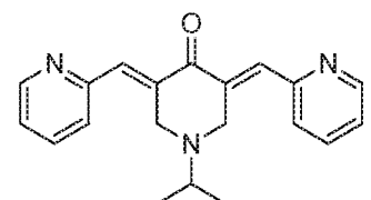
SYC-916 (Compound 7-9)
