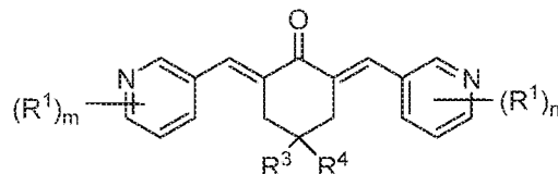
Structure I-B3
