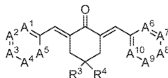
Structure I-B
