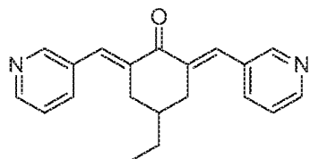
SYC-944 (Compound 2-8) (or MCB-613)
