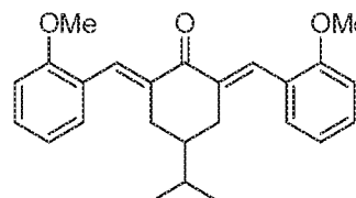
SYC-972 (Compound 8-1)
