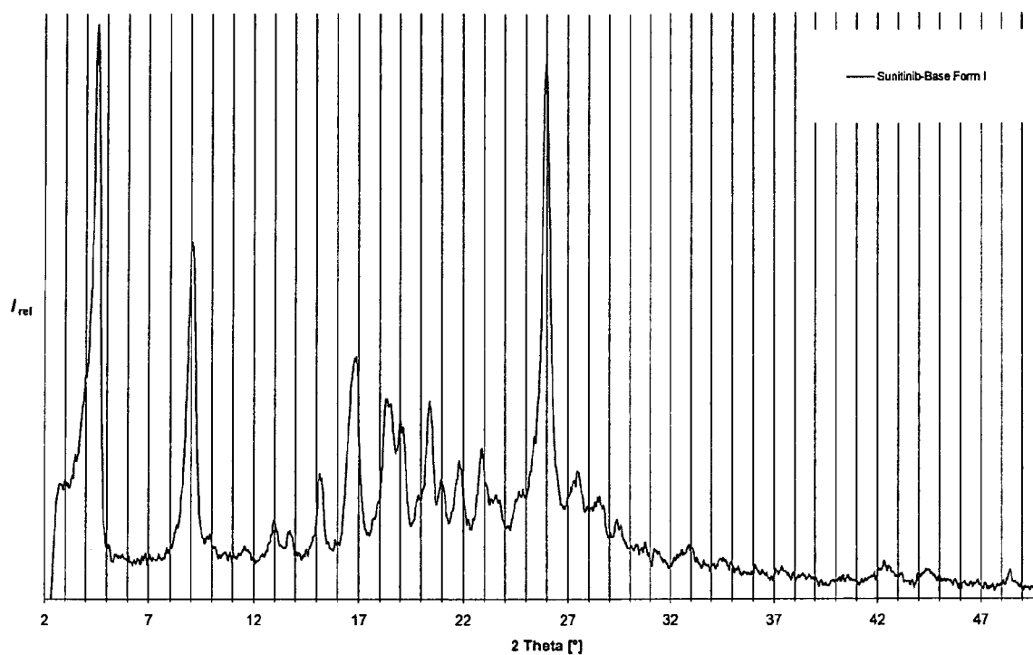
Figure 1: XRPD pattern of polymorph I of Sunitinib
