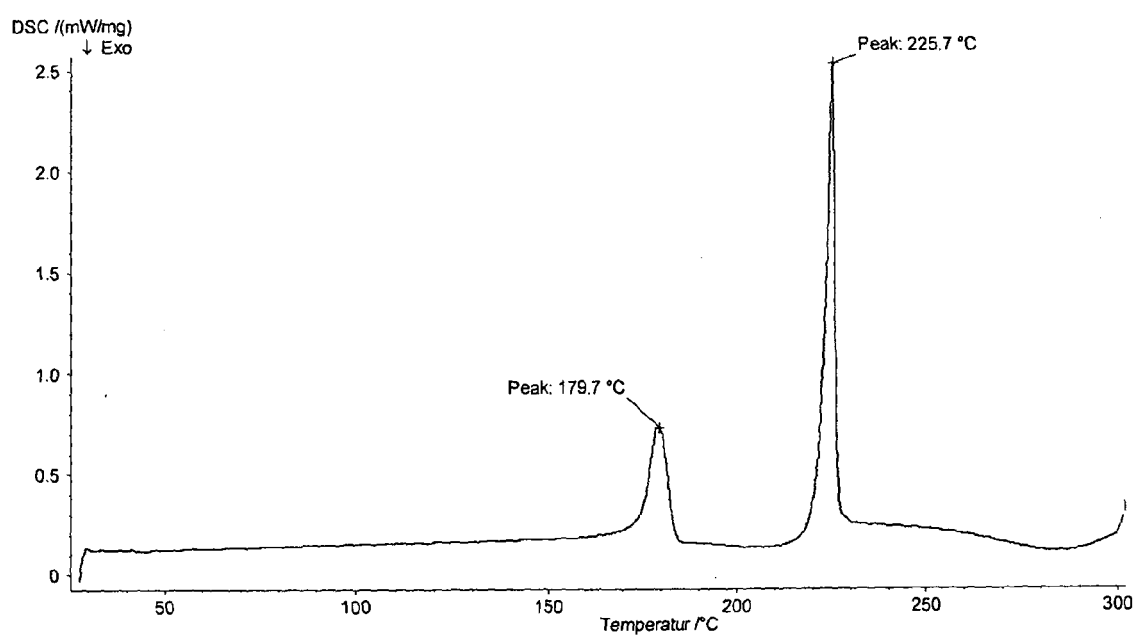
Figure 6: DSC thermogram of polymorph III of Sunitinib
