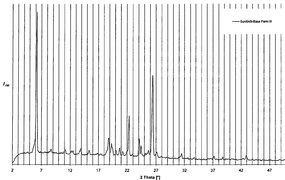
Figure 3: XRPD pattern of polymorph III of Sunitinib
