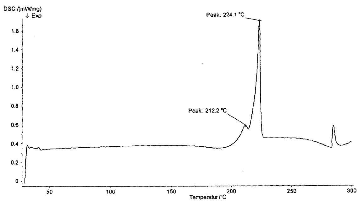
Figure 5: DSC thermogram of polymorph II of Sunitinib
