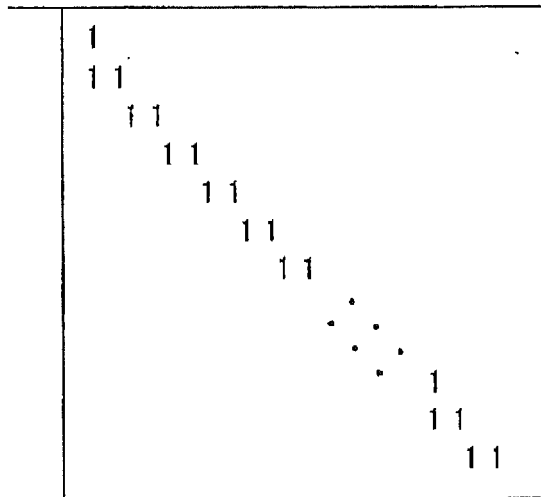
STAIRCASE STRUCTURE OF PARITY MATRIX
