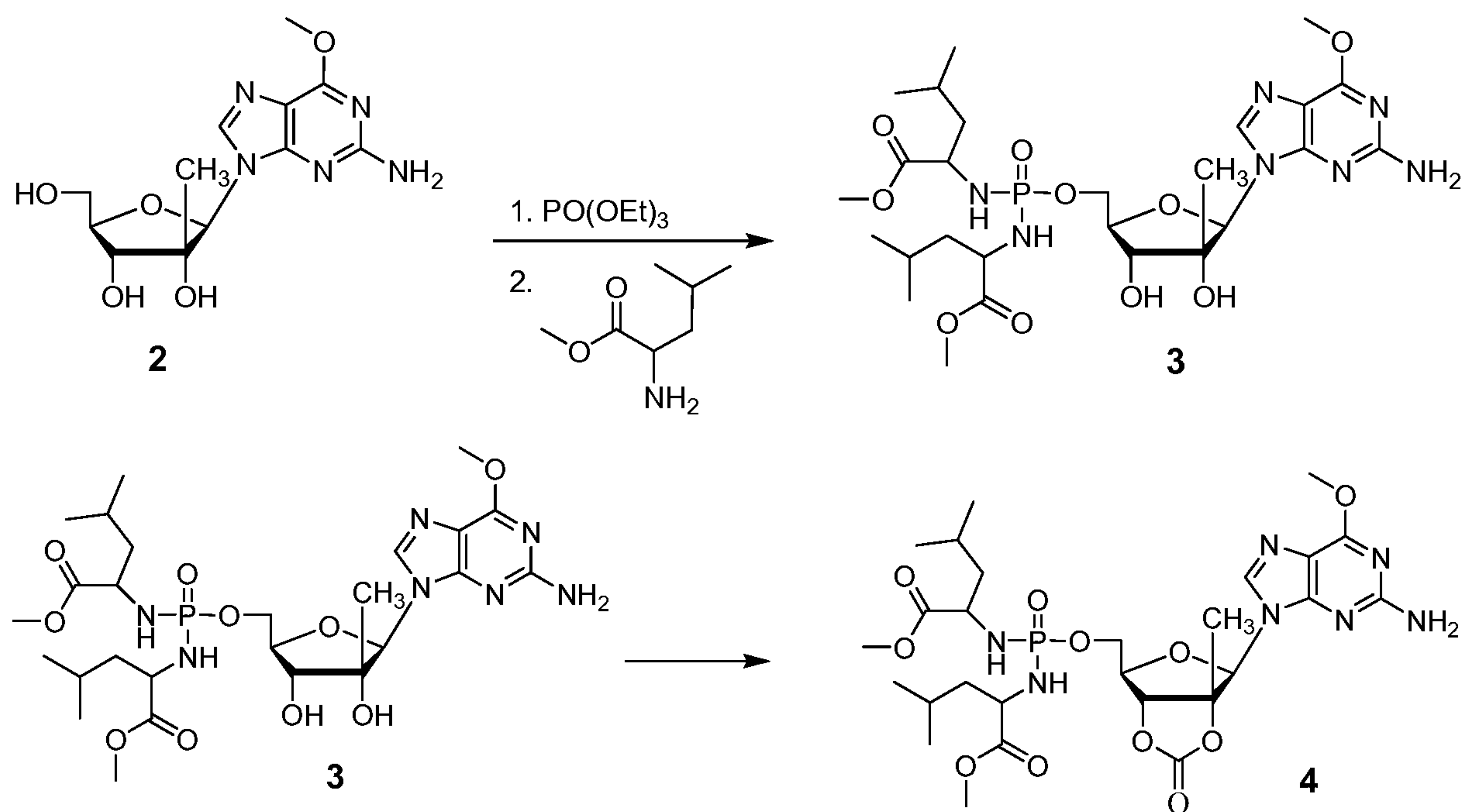
Scheme 4
