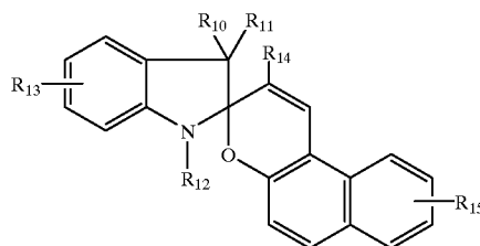
benzothiazoline spiro pyrans
