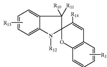
indoline naphtho pyrans
