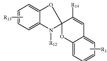
benzoxazoline spiro pyrans
