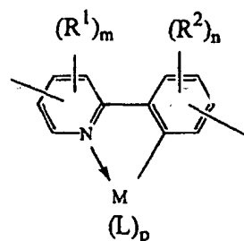
General formula (1)
