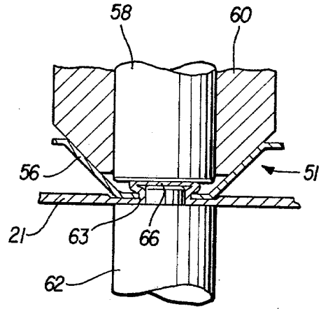
PRIOR ART FIG. 12
