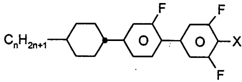
CGU-n-X
