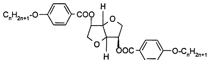
(nOPZ)2X*
