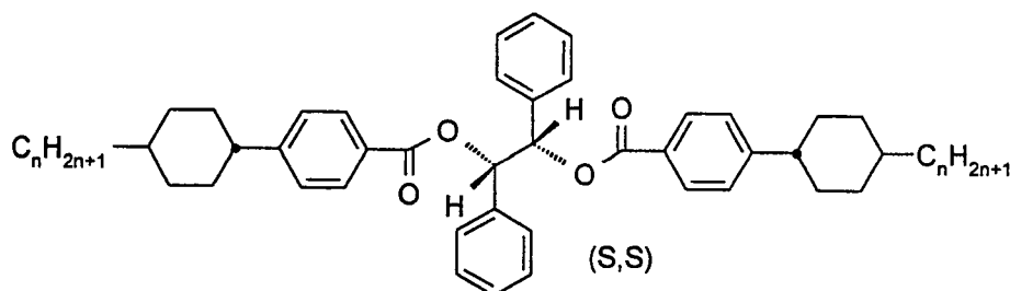
SS-(nCPZ)2BE
