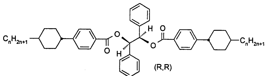
RR-(nCPZ)2BE
