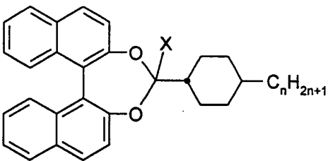
BO2C*F-C-n
