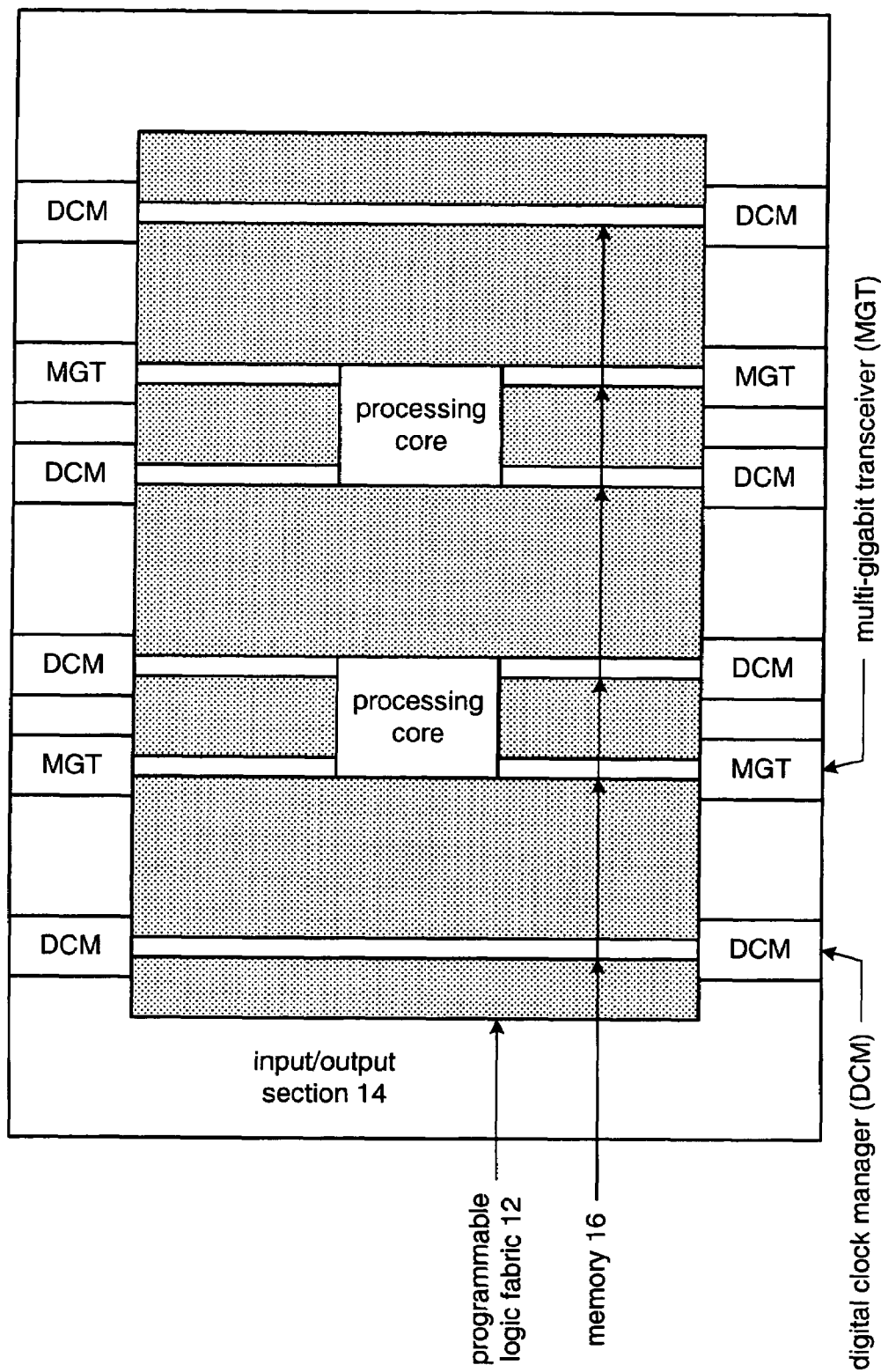
FIG. 1 programmable logic device 10
