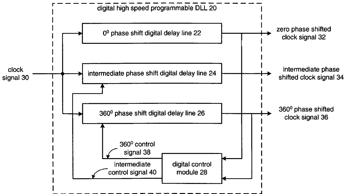
digital clock manager
