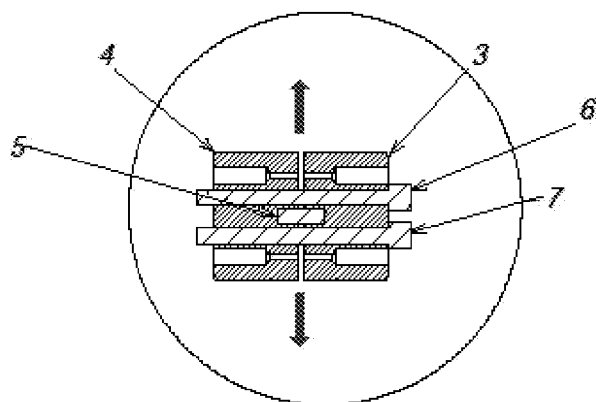
Cross sectional view taken along line 6'-6'
