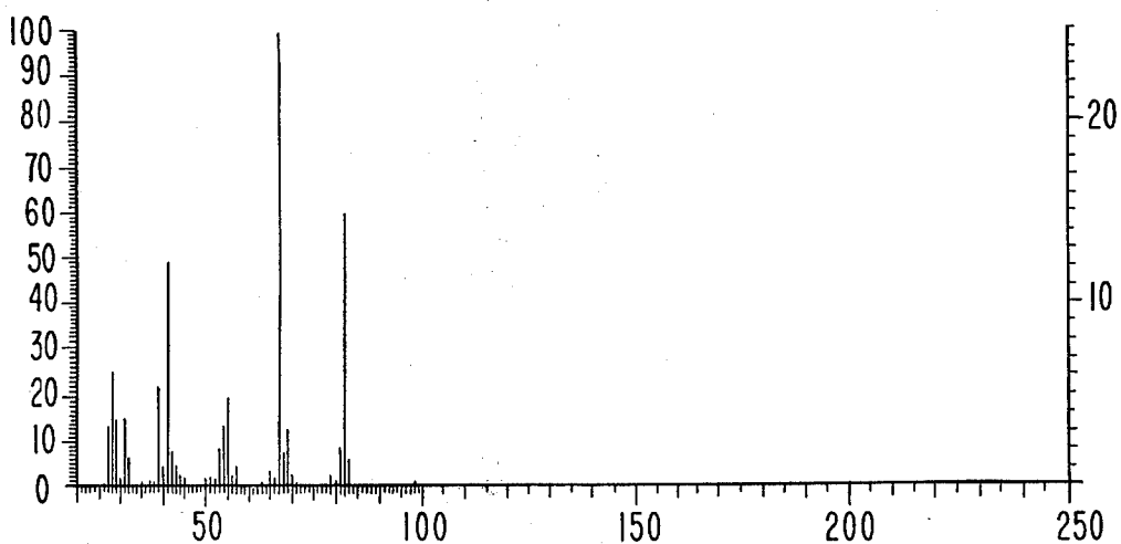
MASS SPECTRUM FOR EXAMPLE II.
