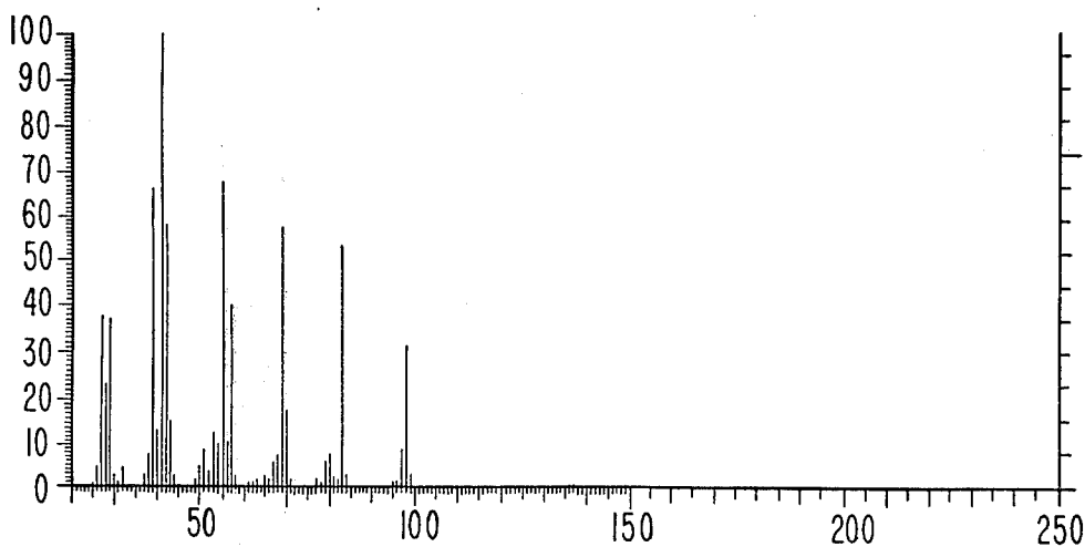
MASS SPECTRUM FOR EXAMPLE II.
