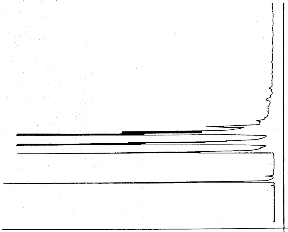
FIG.14 GLC PROFILE FOR EXAMPLE III.
