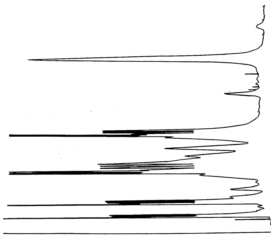
FIG. 1 GLC PROFILE FOR EXAMPLE I
