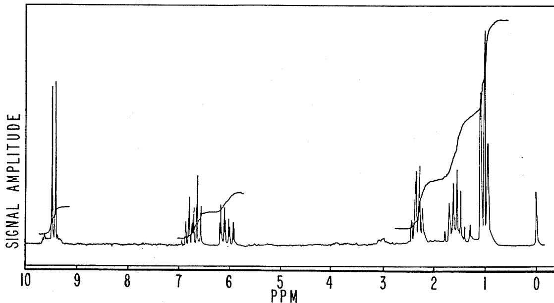
NMR SPECTRUM FOR EXAMPLE II.
