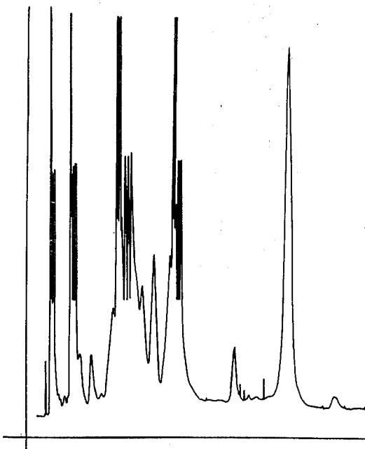
GLC PROFILE FOR EXAMPLE I
