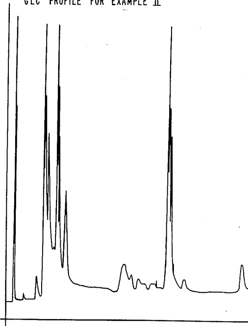
GLC PROFILE FOR EXAMPLE II
