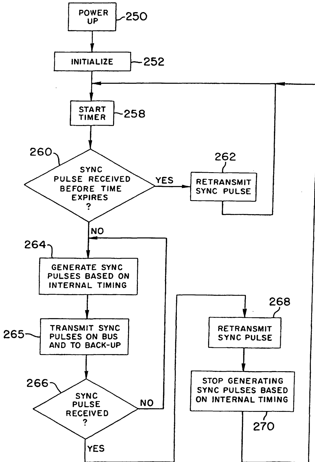
FIG. 10A (HYBRID-MASTER)
