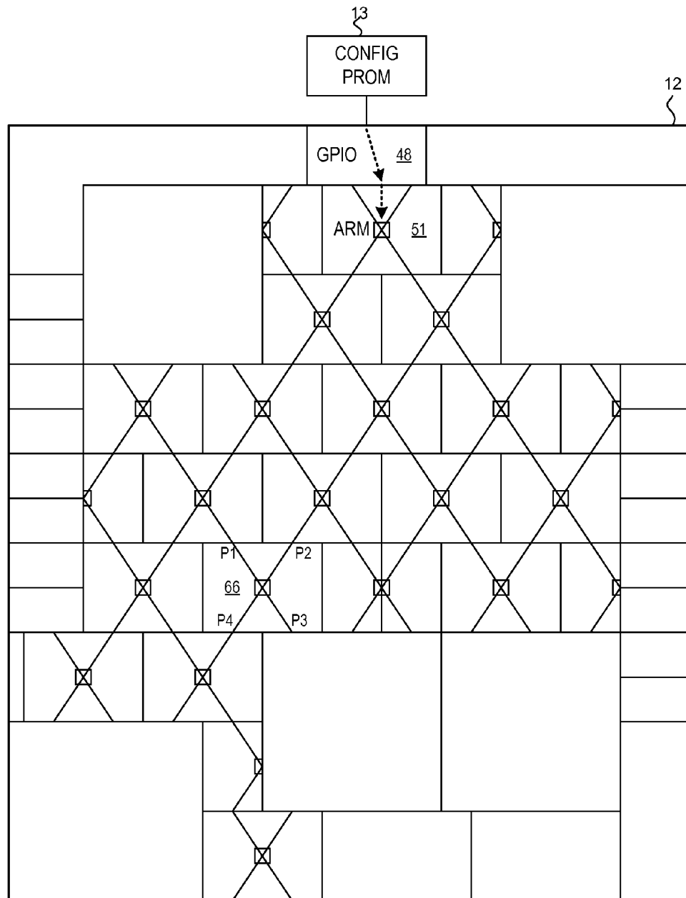
CONFIGURABLE MESH CONTROL BUS STRUCTURE
