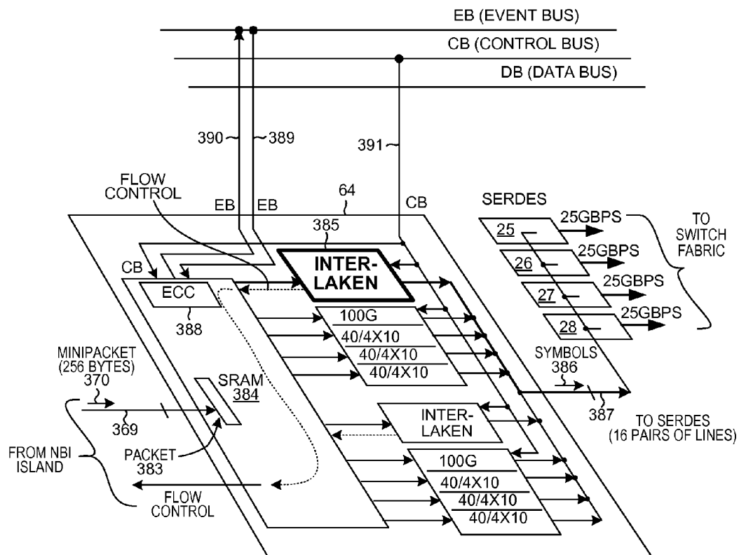
MAC ISLAND (EGRESS)
