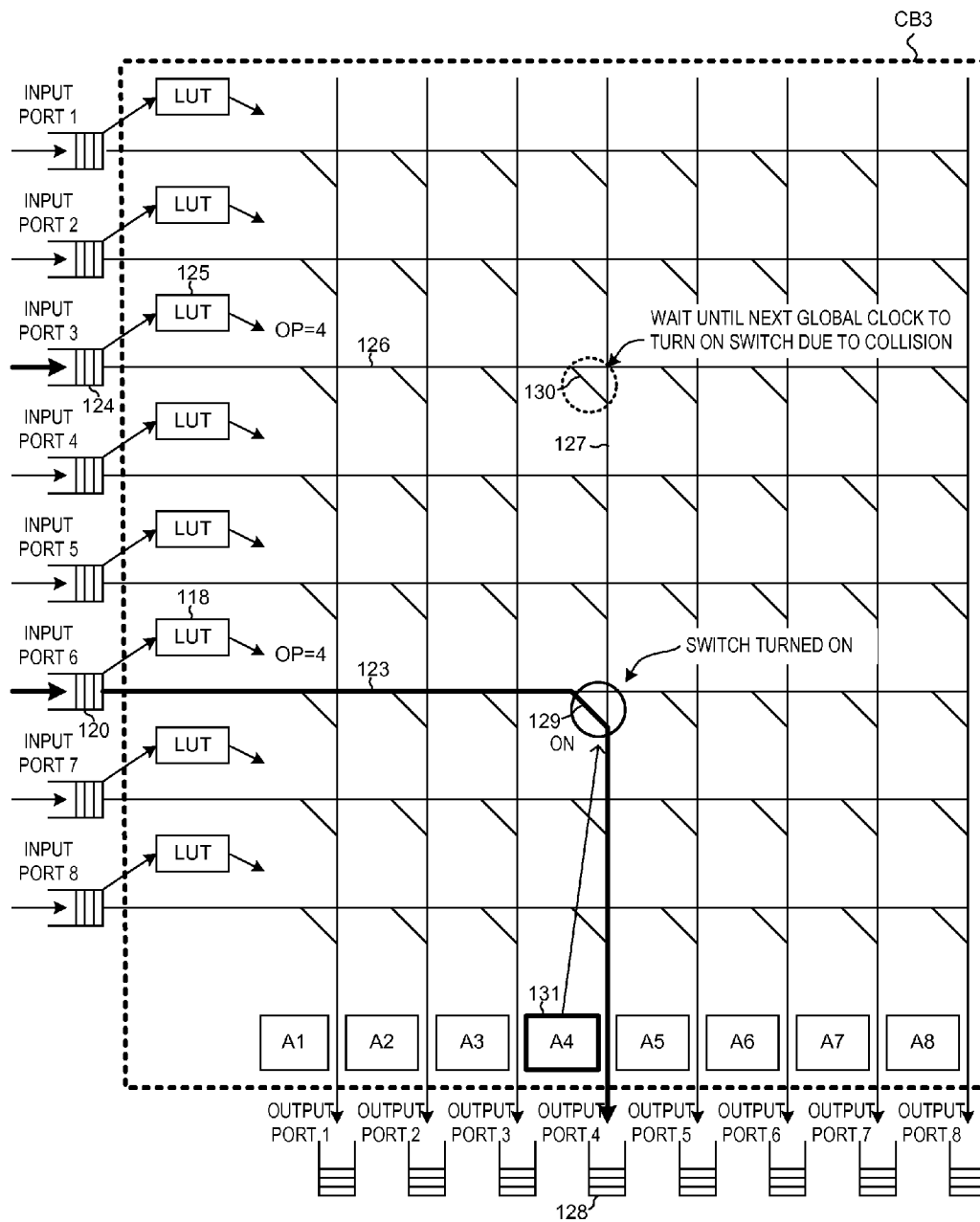
8-WAY CROSSBAR SWITCH FIG. 13
