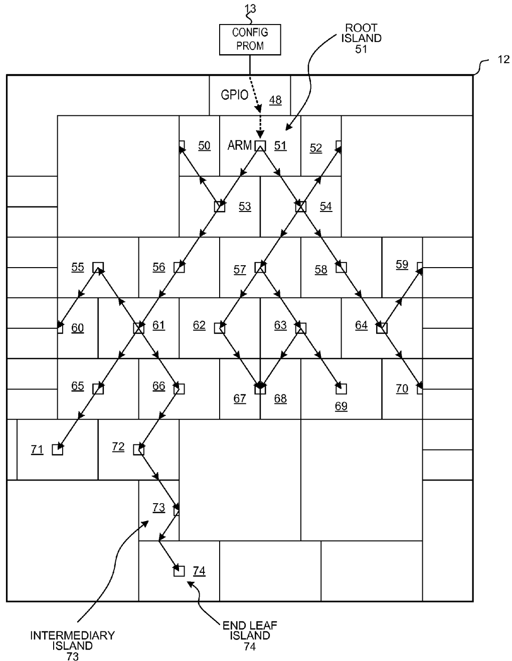
CONFIGURED CONFIGURABLE MESH CONTROL BUS
