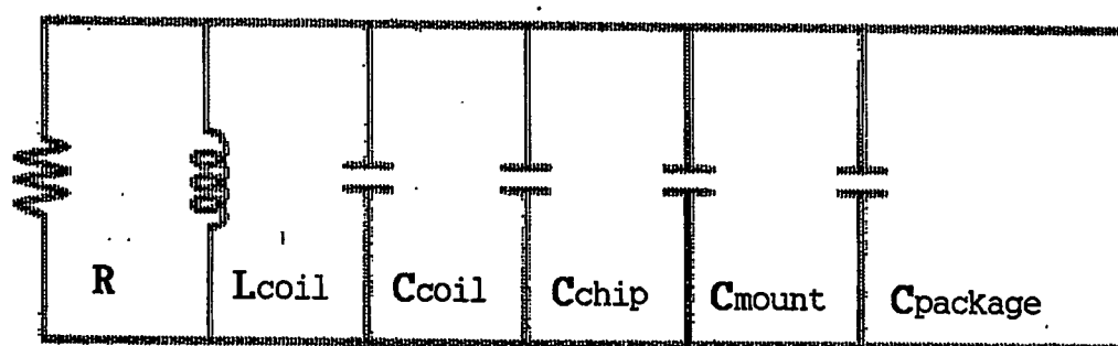
EQUIVALENT CIRCUIT OF THE CONVENTIONAL SMART CARD OF A COMBINATION TYPE
