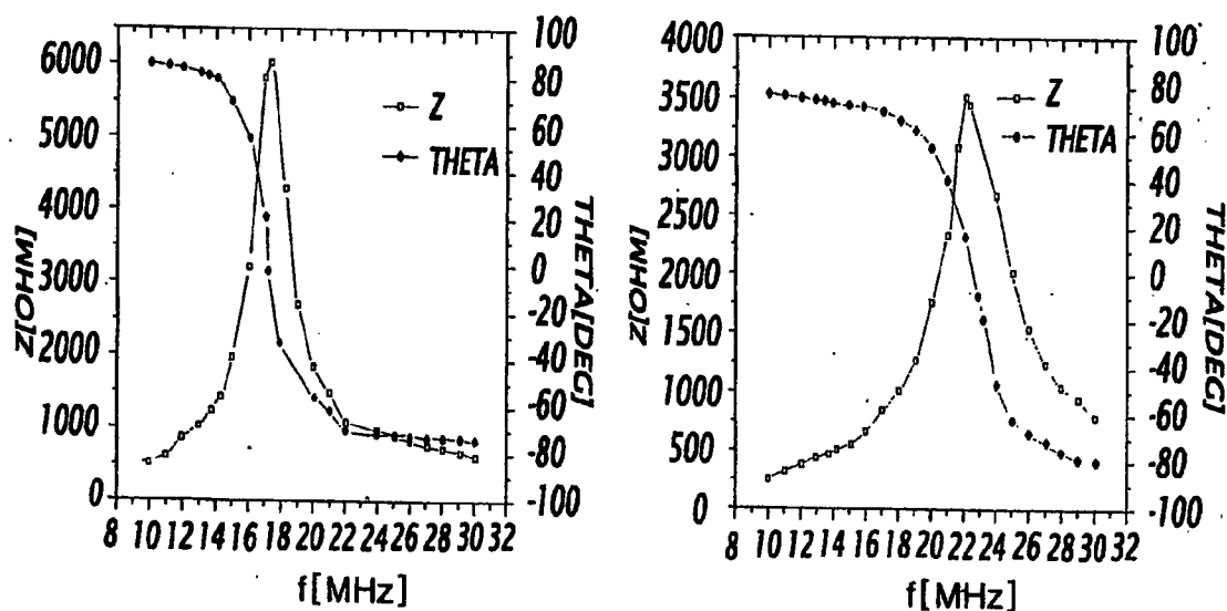
(a) BEFORE TESTING (b) AFTER TESTING GRAPH OF IMPEDANCE-FREQUENCY CHARACTERISTICS IN THE CONVENTION SMART CARD OF A COMBINATION TYPE
