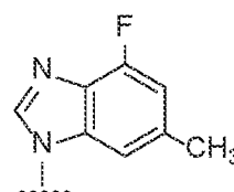
4-Fluoro-6- methylbenzimidazole
