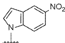
5-nitroindole
