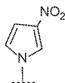
3-nitropyrrole
