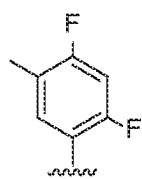
2,4- difluorotoluene
