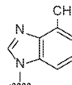
4-Methylbenzimidazole
