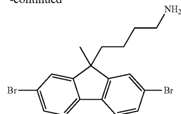
Step 3: 4-(2,7-dibromo-9-methyl-9H-fluoren-9-yl)butan-1-amine
