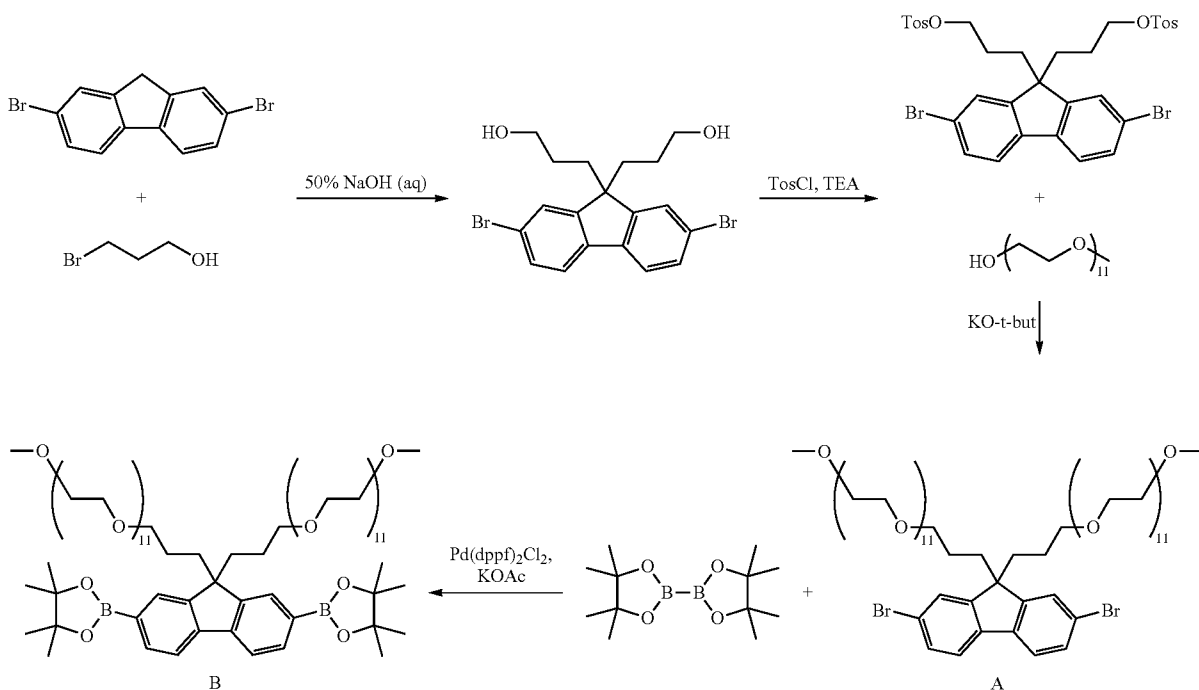
Step 1: 2,7-dibromo-9,9-di(3'-hydroxypropyl)fluorene
