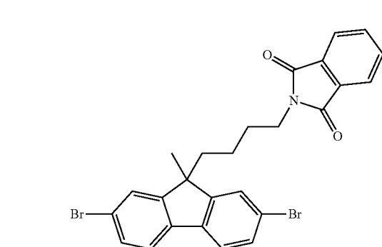
Step 2: 2-(4-(2,7-dibromo-9-methyl-9H-fluoren-9-yl)butyl)isoindoline-1,3-dione
