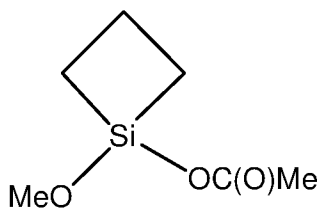
1-methoxy-1-acetoxy-1-silacyclobutane
