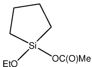
1-ethoxy-1-acetoxy-1-silacyclopentane
