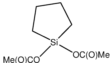
1,1-diacetoxy-1-silacyclopentane
