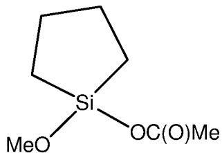
1-methoxy-1-acetoxy-1-silacyclopentane
