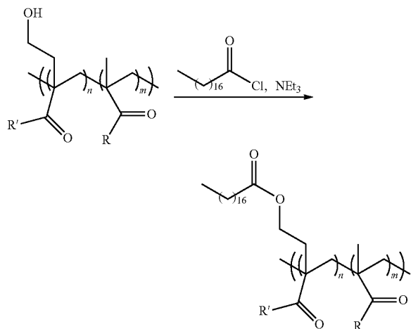
Reaction Scheme 6
