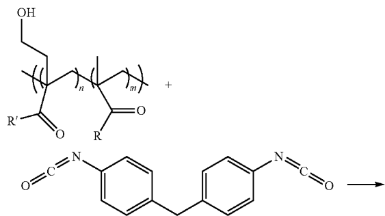
Reaction Scheme 3
