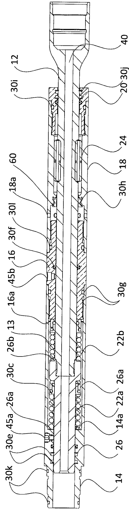
TOOL IN FULL EXTENSION
