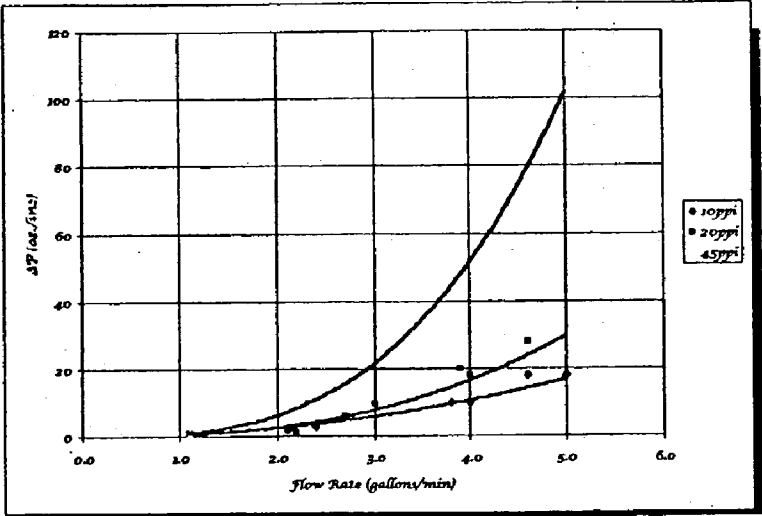
Figure 31: Relationship of Flow Rate of Water and Pressure Drop
