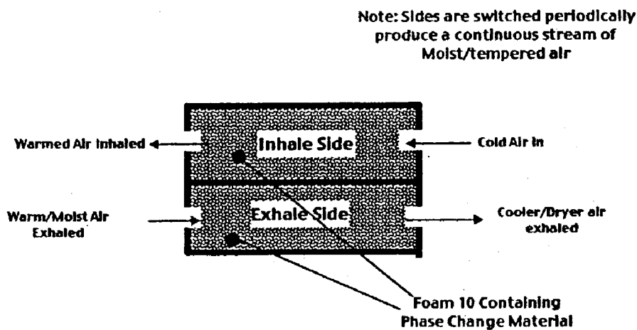
Figure 28: Respirator
