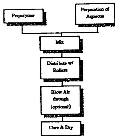
Figure 8: Process to Manufacture the Composite by the Emulsion Process
