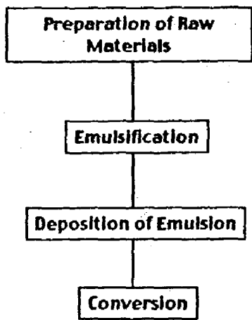
Figure 5: Manufacturing Process for Hydrophilic Polyurethane Foams
