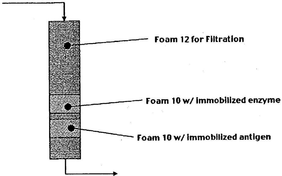
Figure 29: Flow-Through Diagnostic Device
