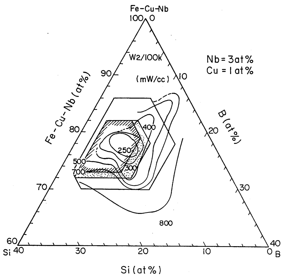
CORE LOSS W 2 /100k OF Fe - Cu 1 - Nb 3 - Si - B ALLOY
