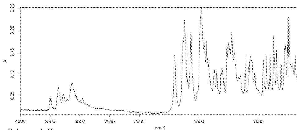
Polymorph II
