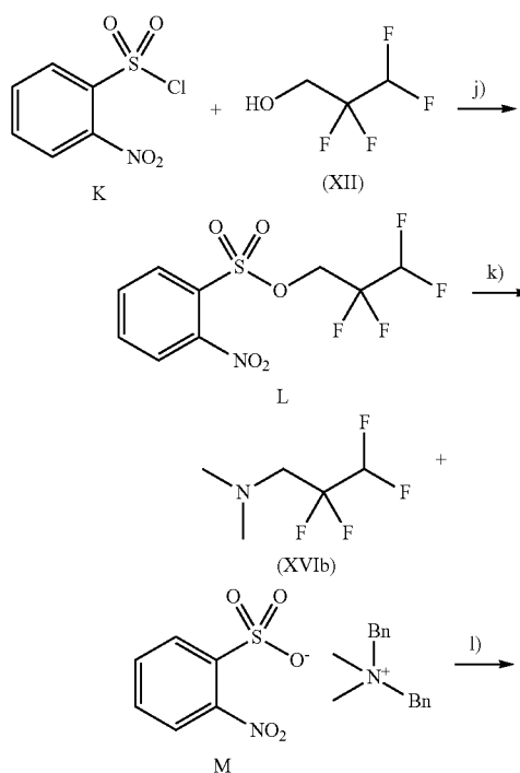
Scheme 4:
