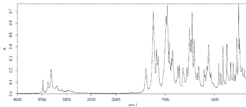
Polymorph III
