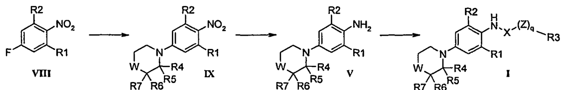
Scheme 4.
