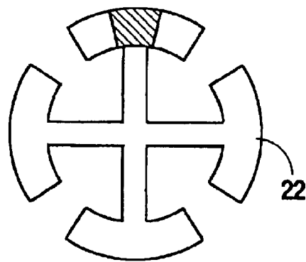
Fig. 5 (SECTION E-E)
