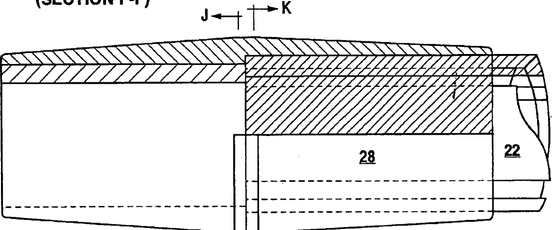
Fig. 6 (SECTION F-F)
