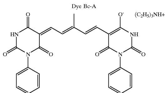
Compound Bc-A
