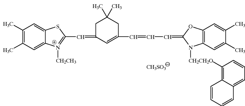
Compound A
