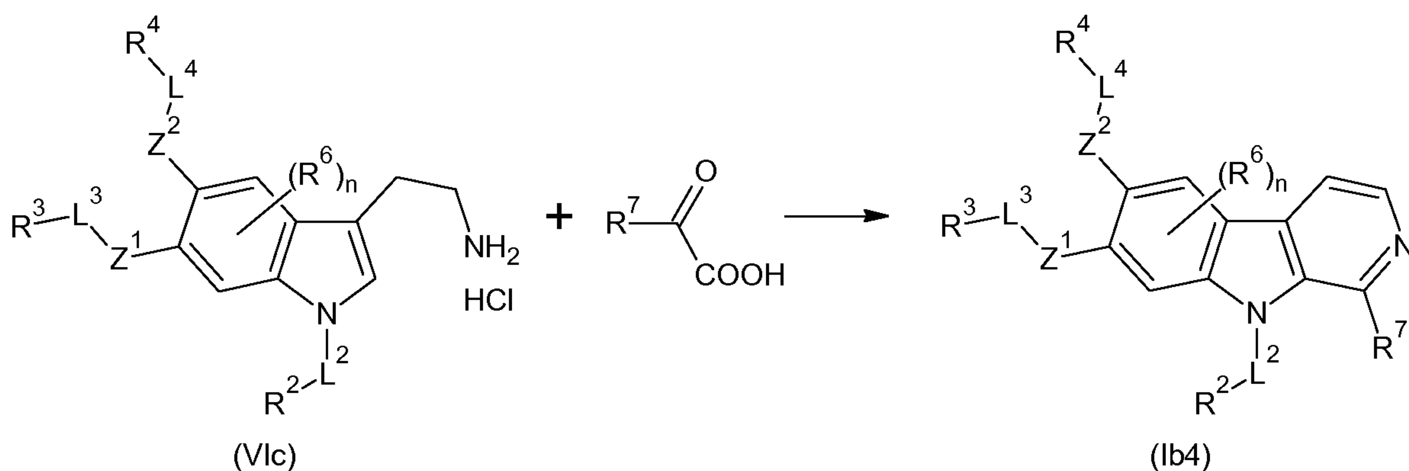
Scheme 9
