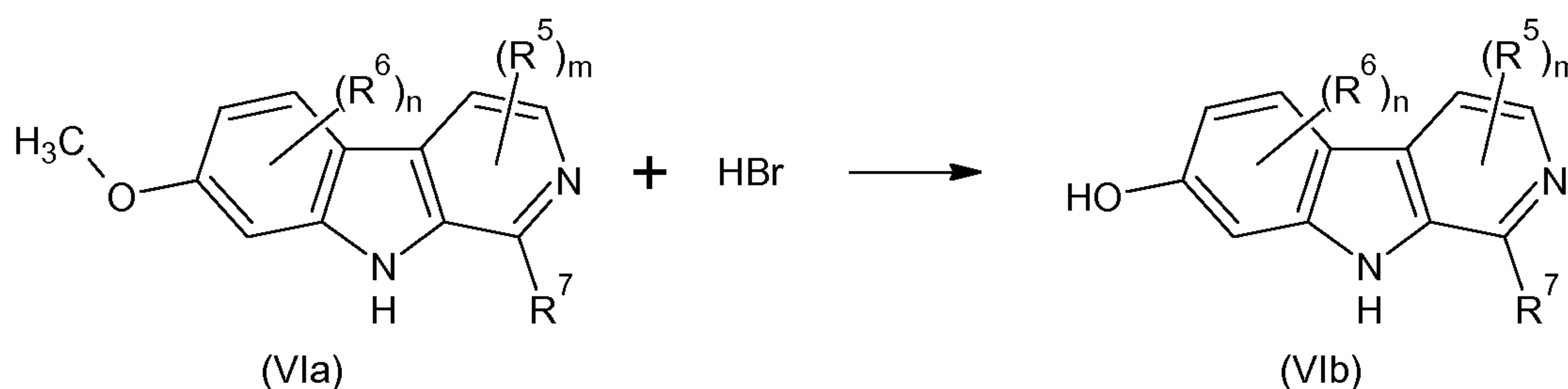
Scheme 3
