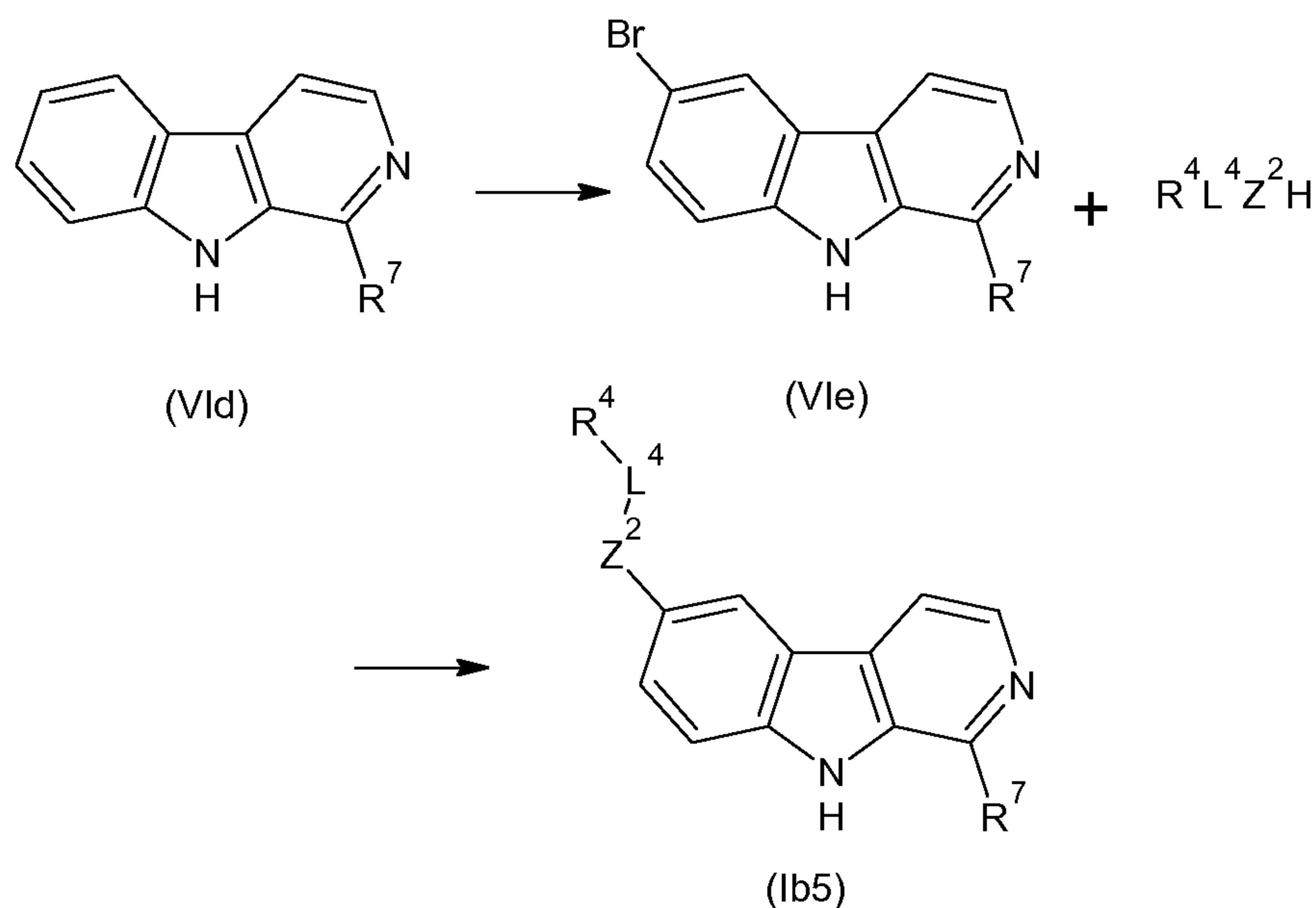
Scheme 10
