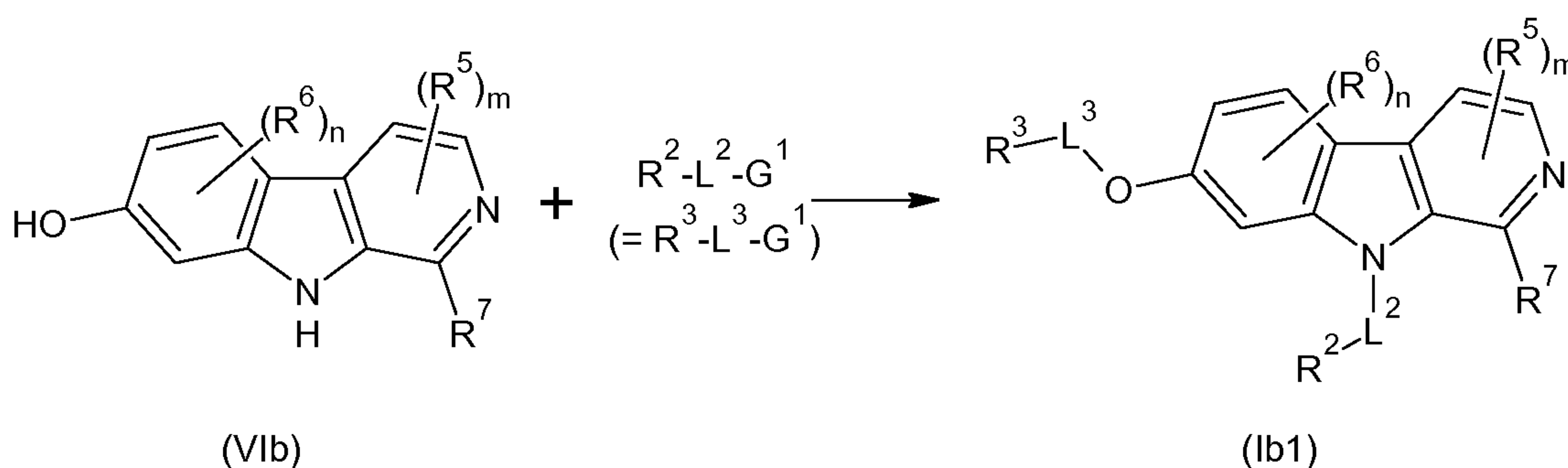
Scheme 2
