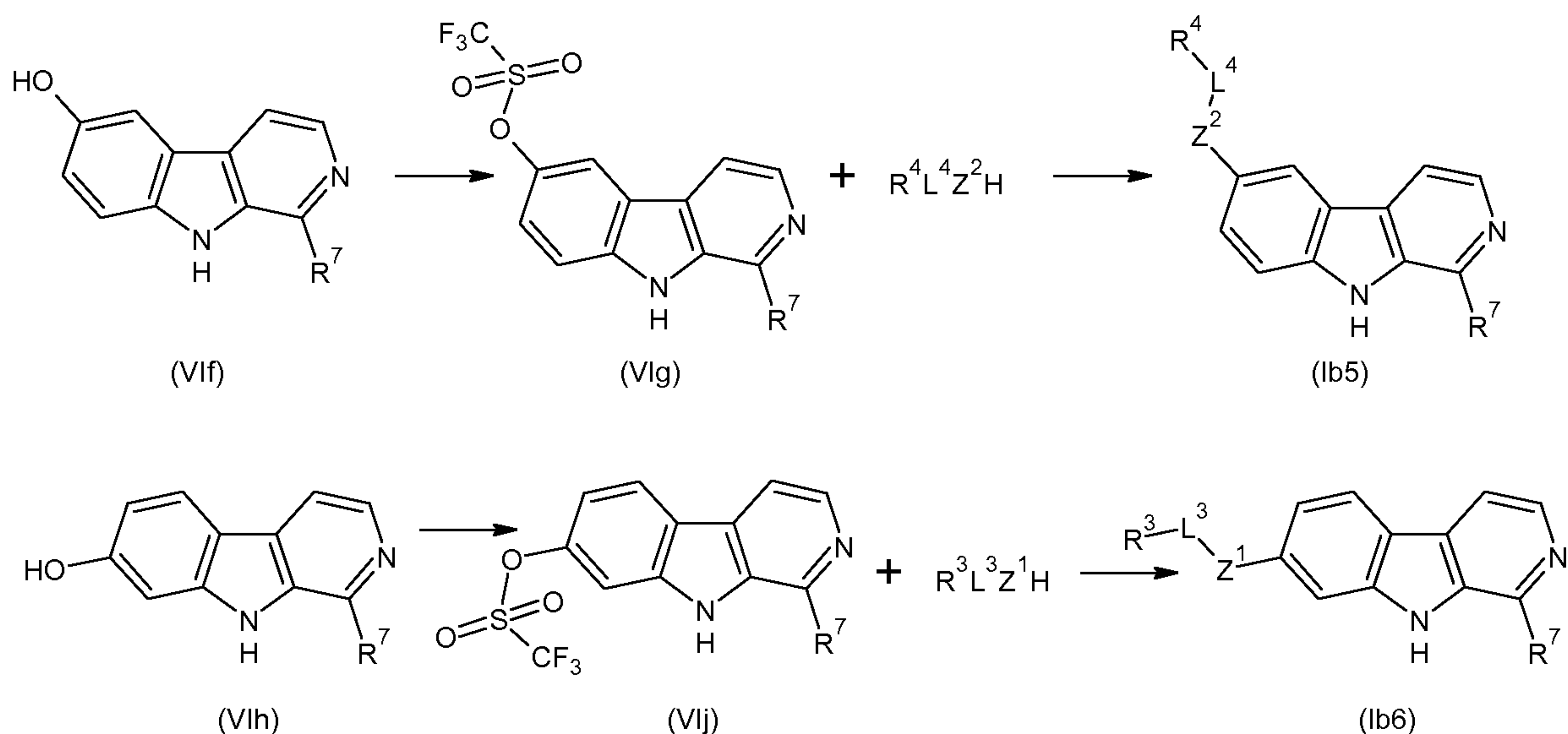
Scheme 11
