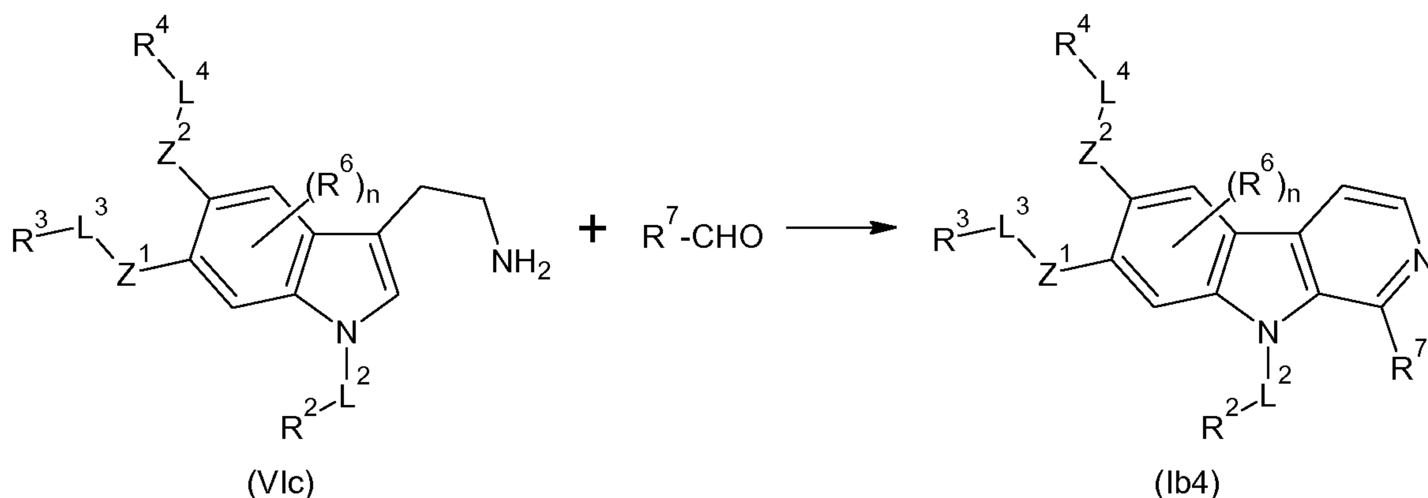
Scheme 8
