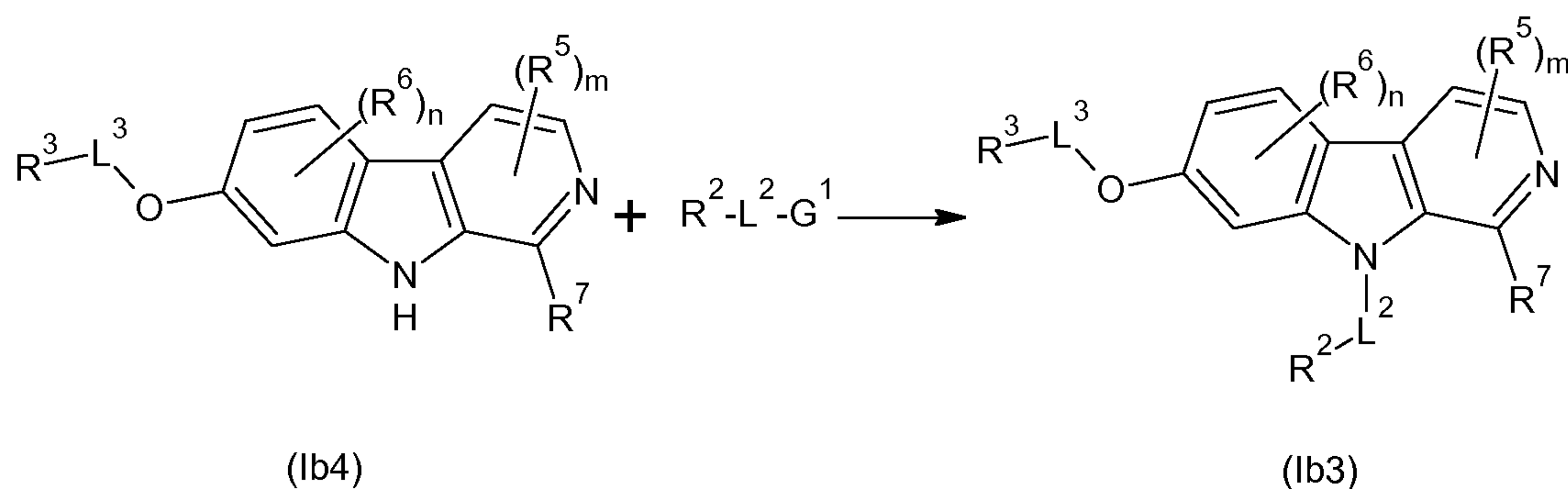
Scheme 15
