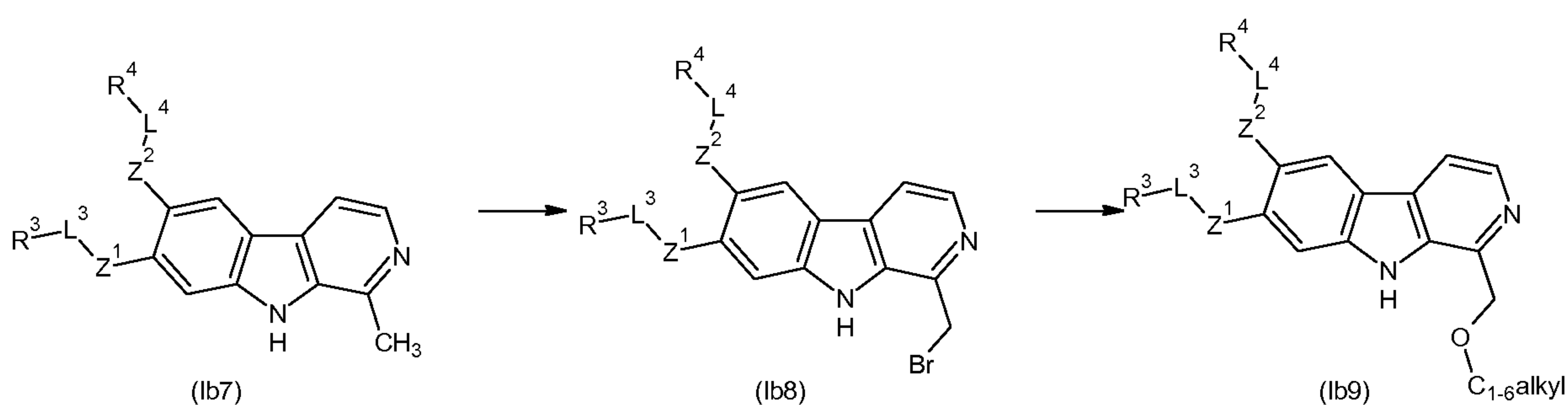
Scheme 12
