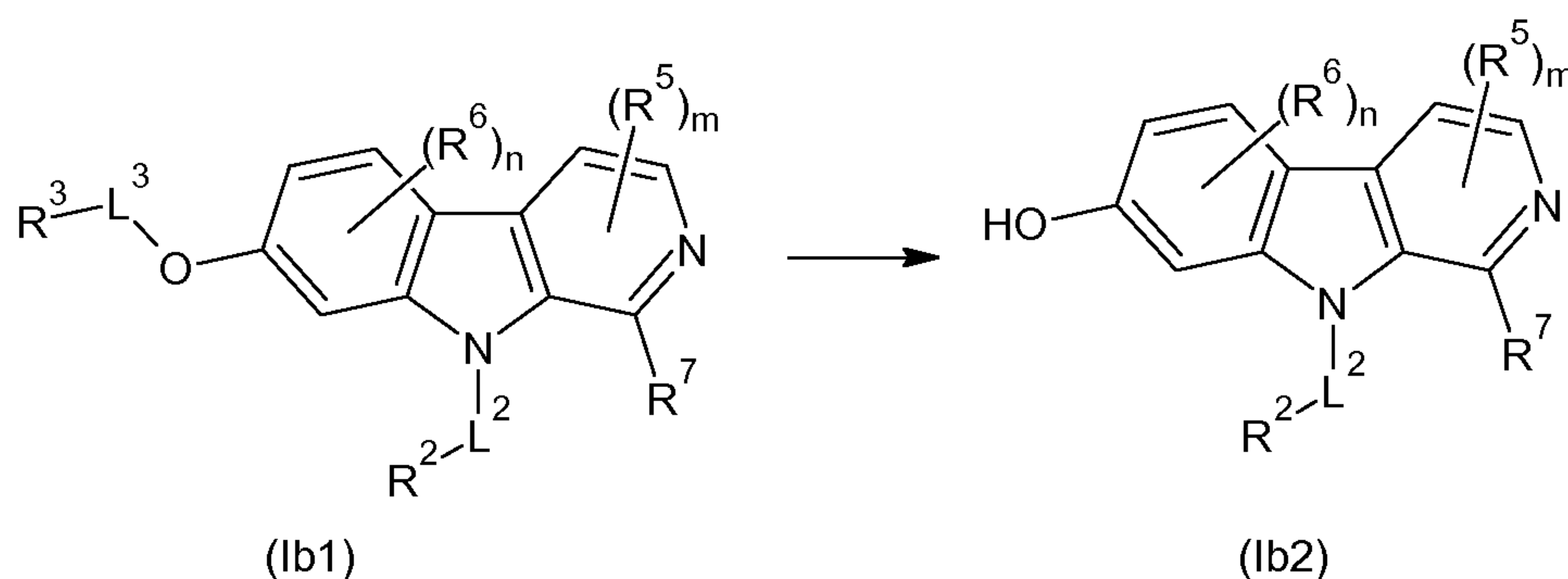
Scheme 13
