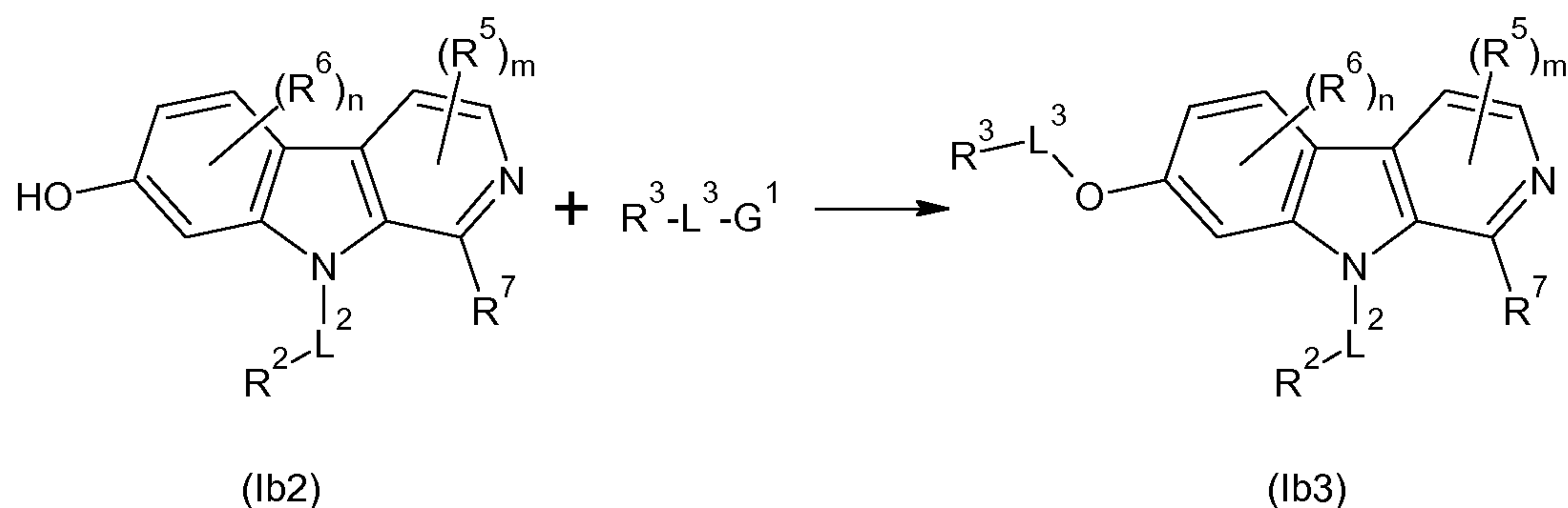
Scheme 6
