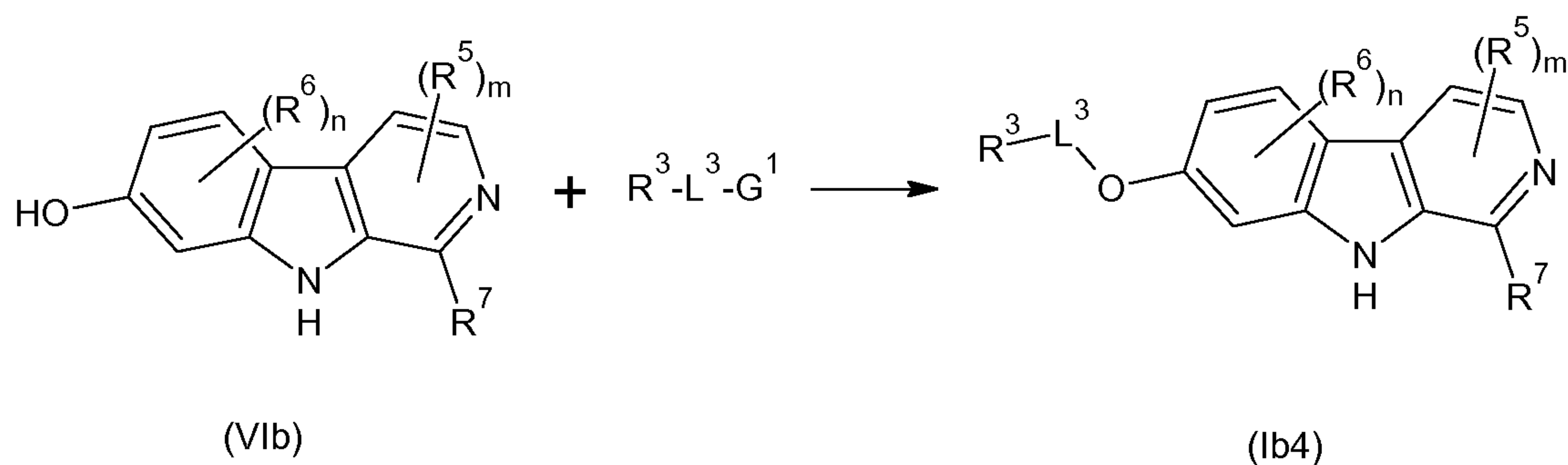
Scheme 14
