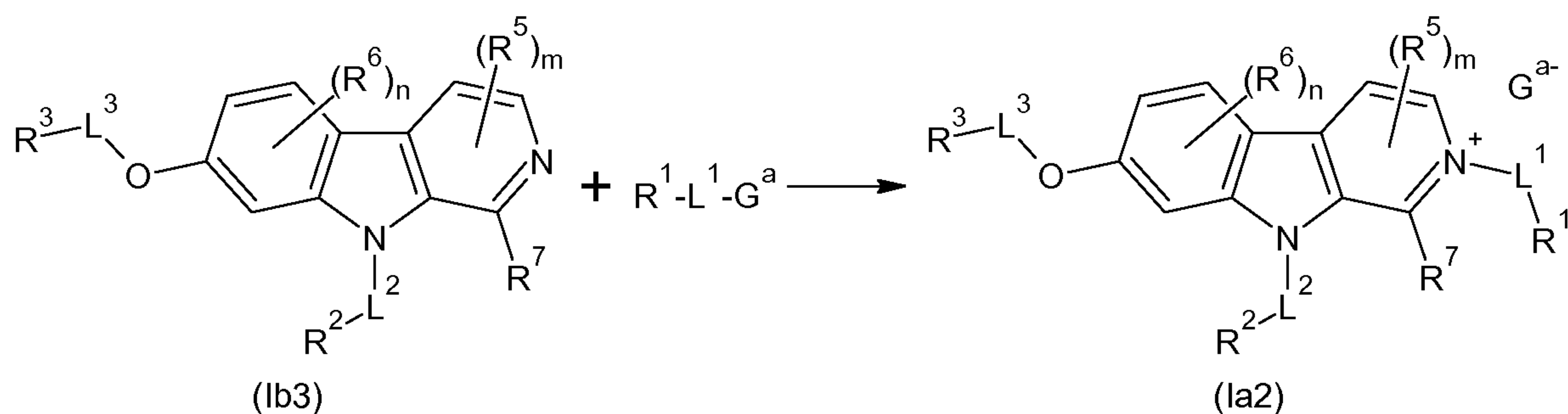
Scheme 7
