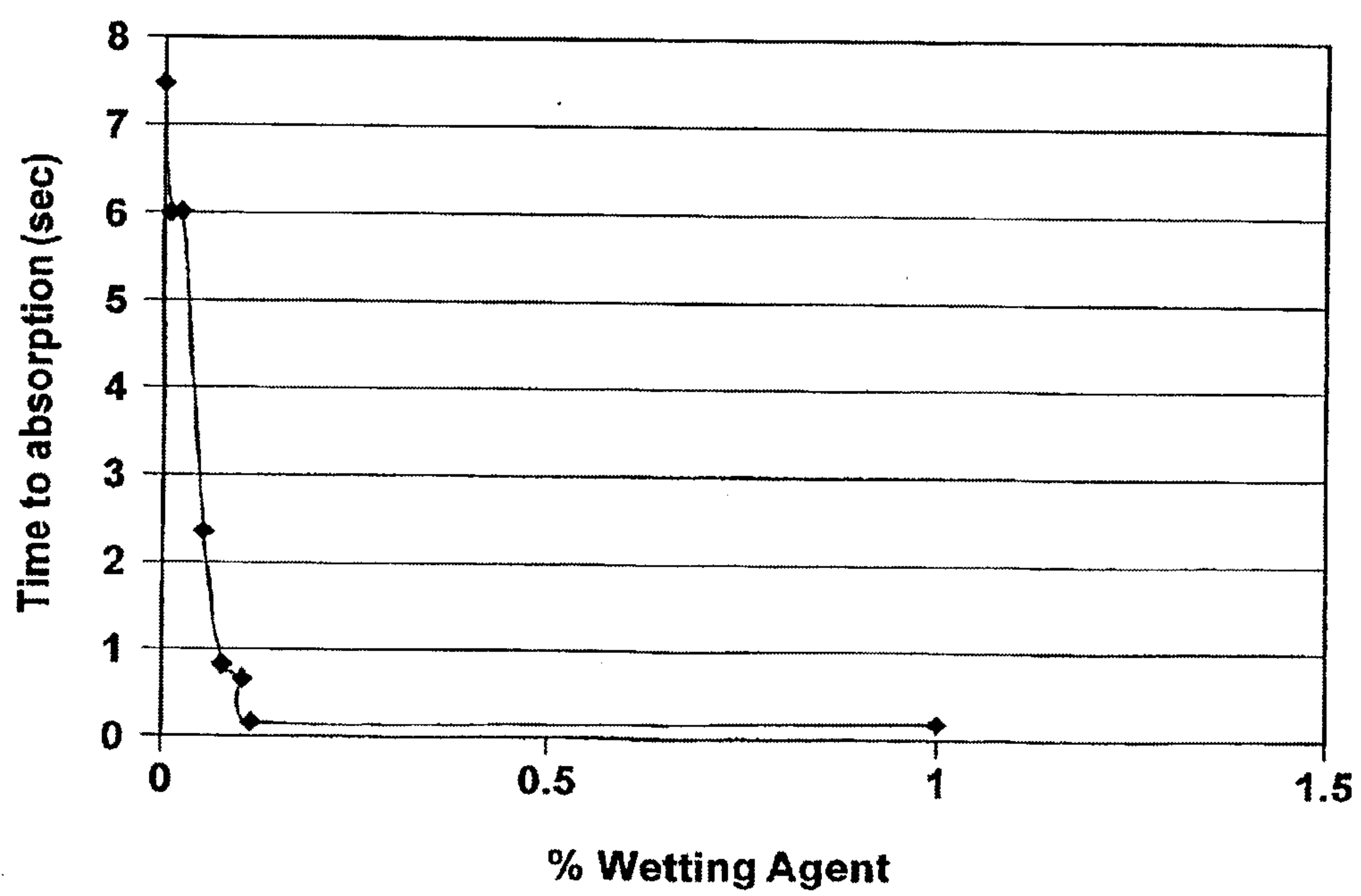
Absorption of water droplet with varying amount of wetting agent
