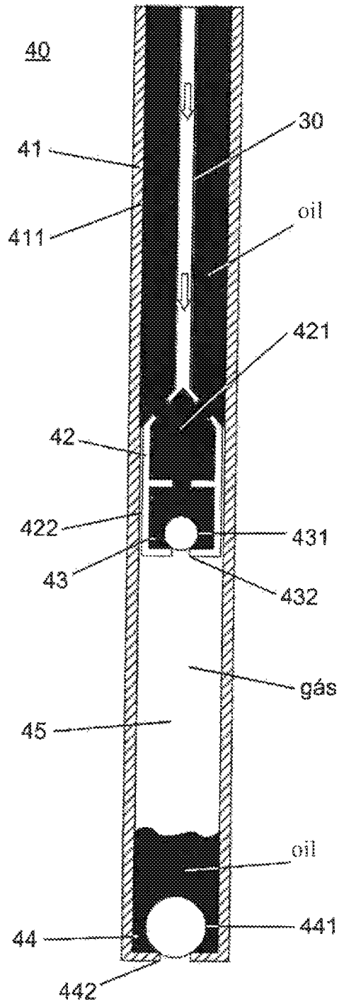
FIG. 5 PRIOR ART
