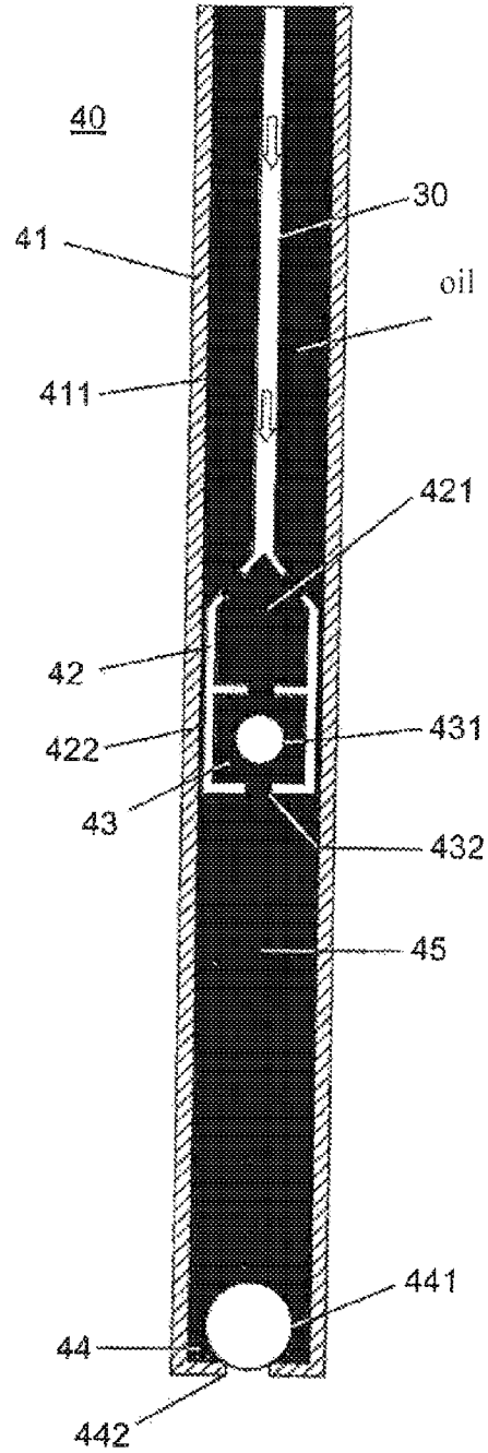
FIG. 3 PRIOR ART
