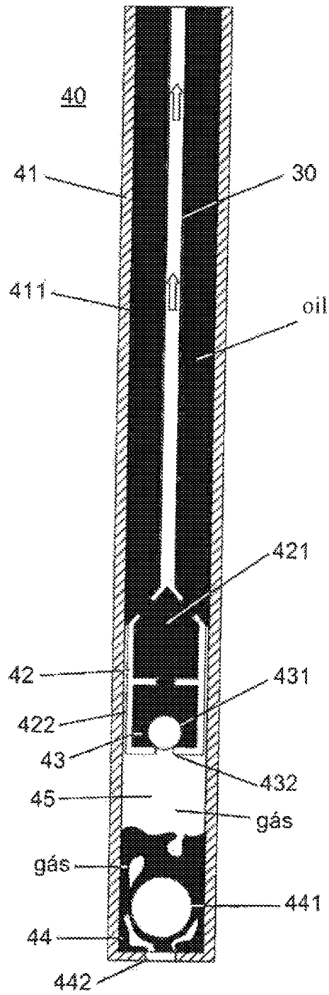
FIG. 4 PRIOR ART
