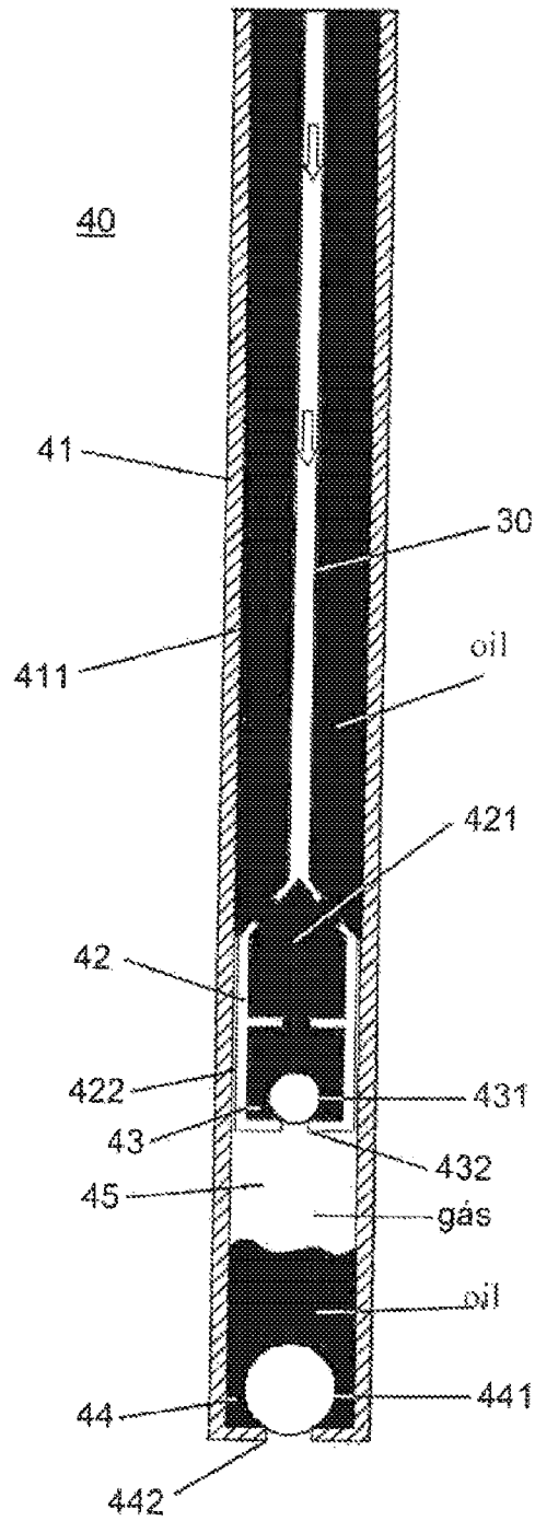
FIG. 6 PRIOR ART
