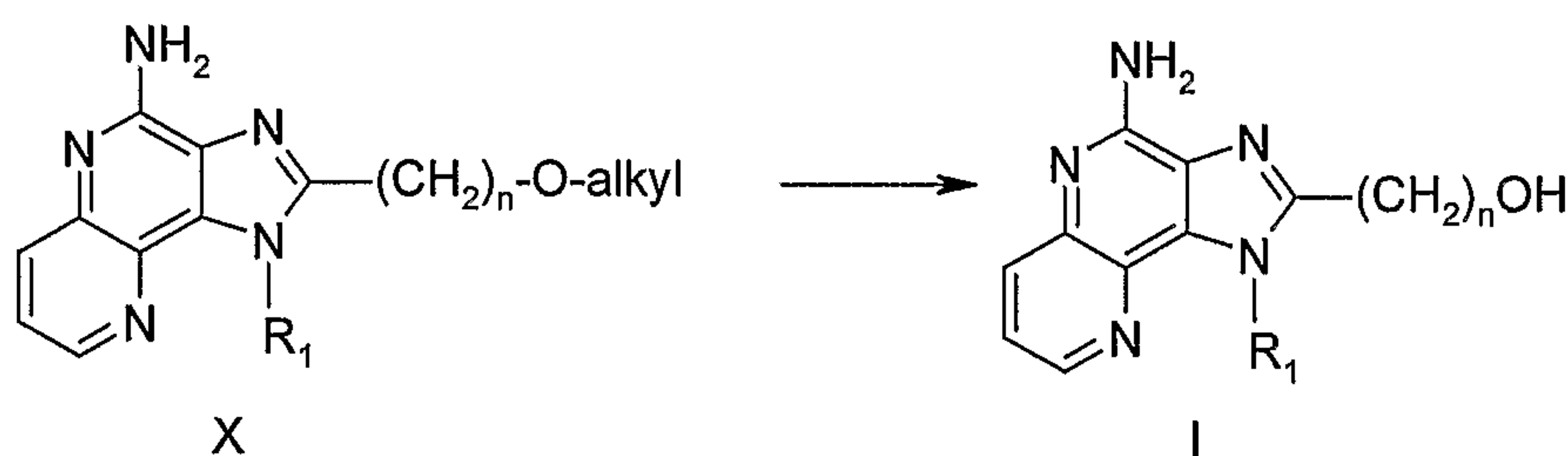
Reaction Scheme I
