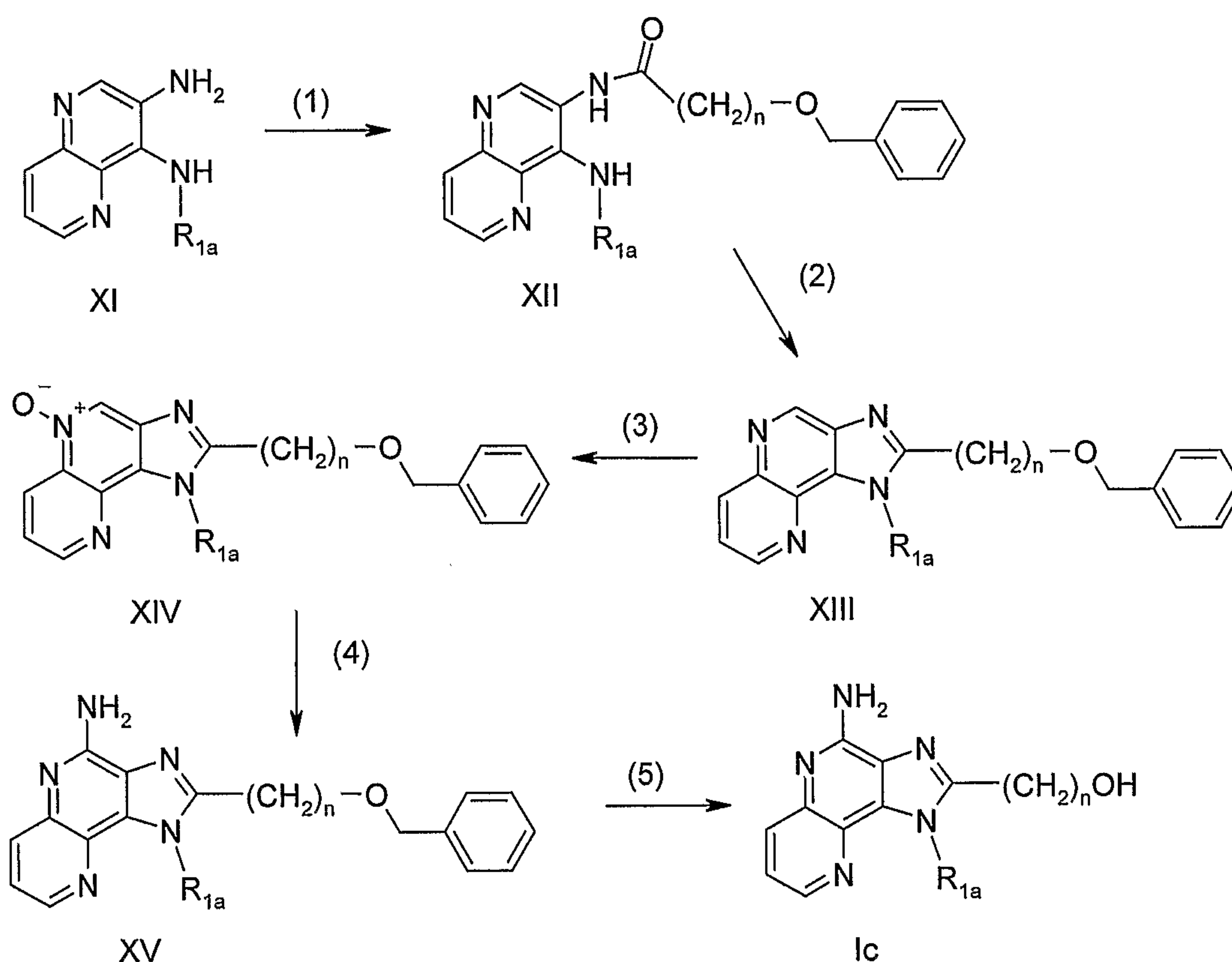
Reaction Scheme II
