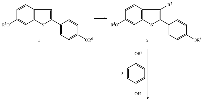
Reaction Scheme I
