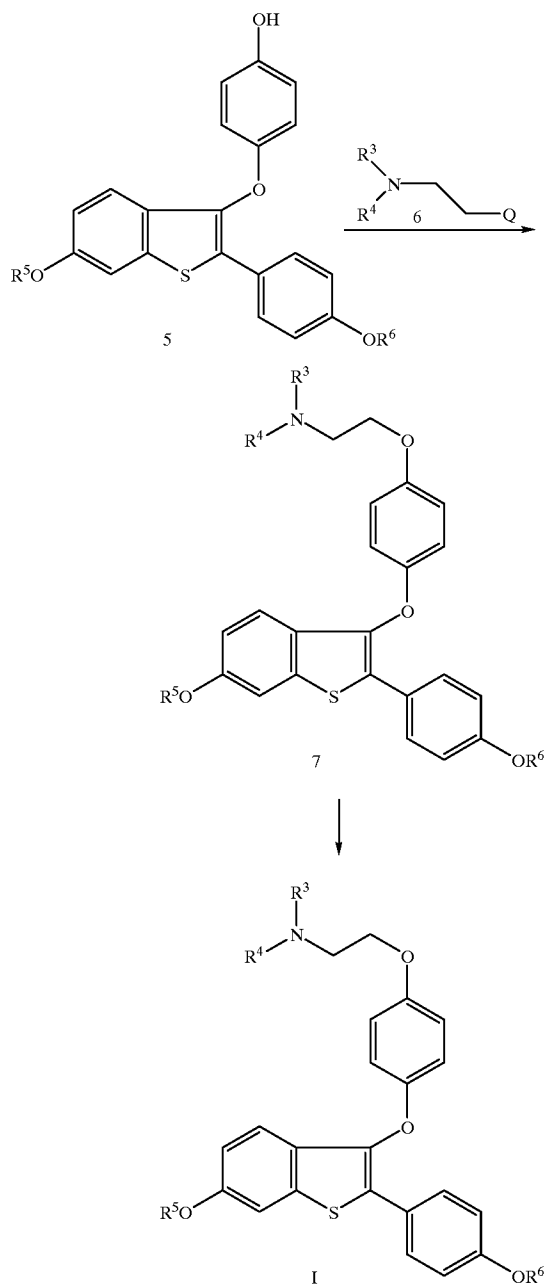
Reaction Scheme II
