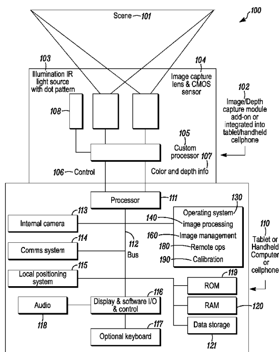
System Block Diagram FIG. 1
