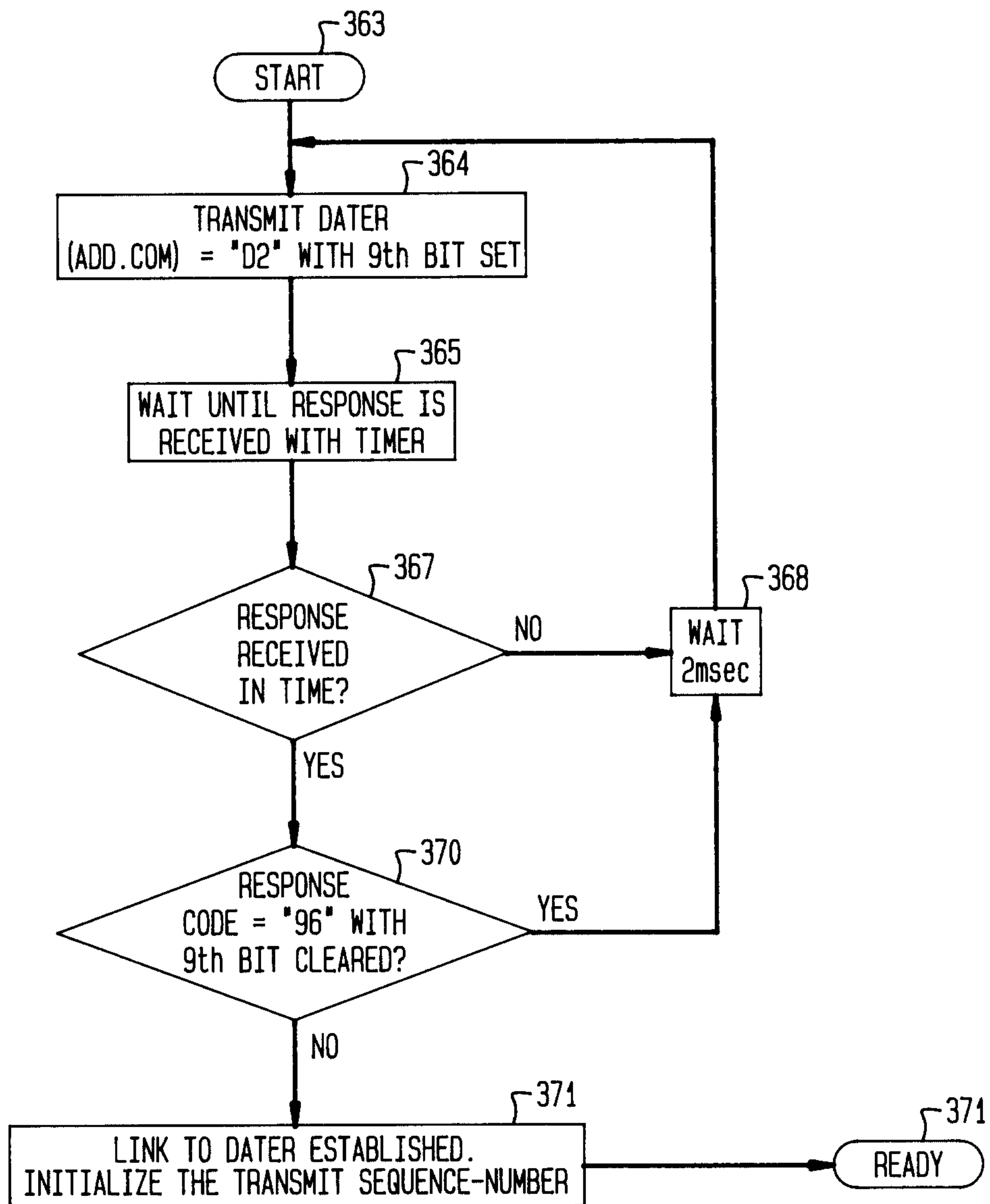
FIG. 9 METER COMMANDS TO LINK DATER
