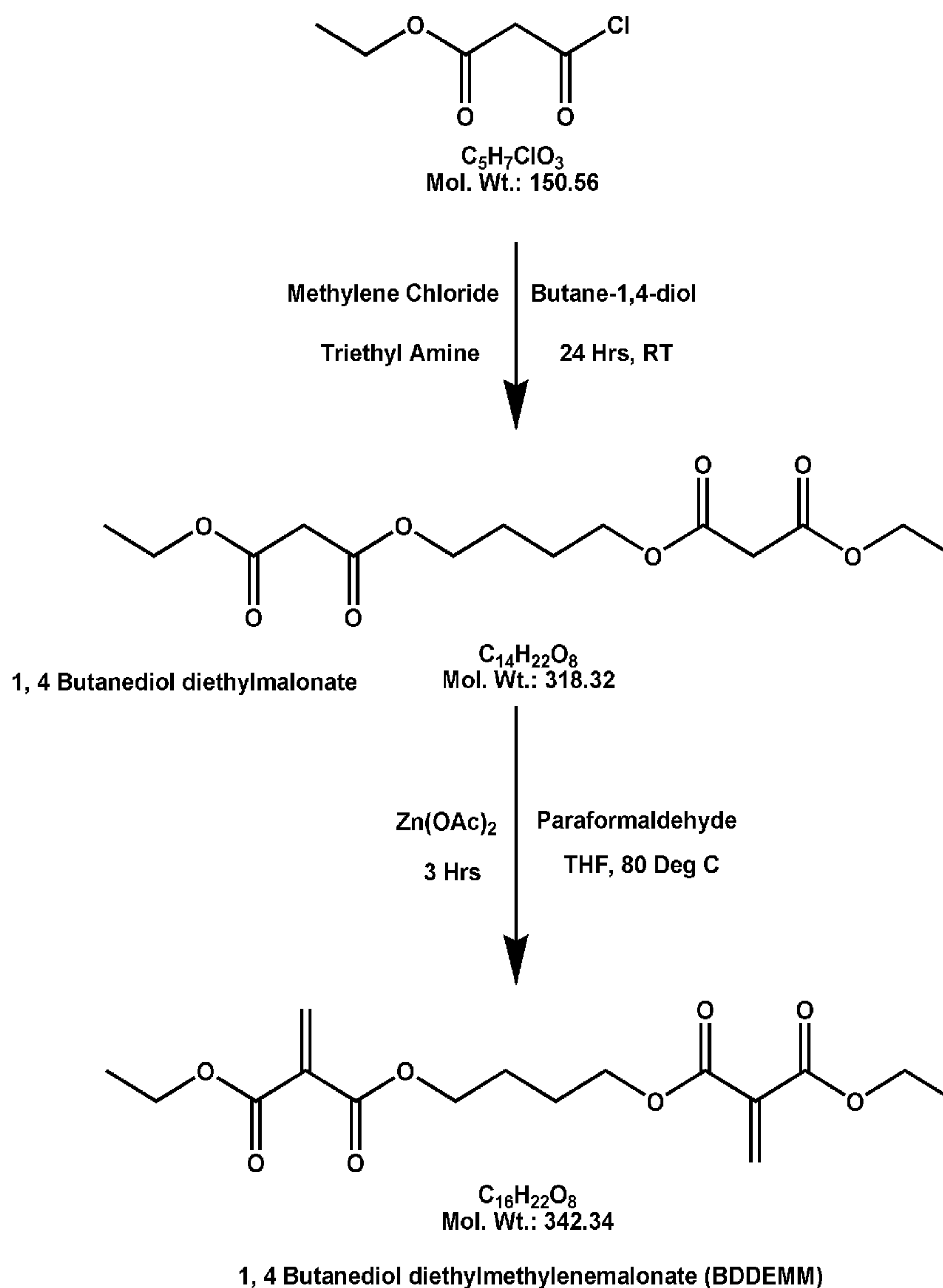
Scheme 1: Formation of MMM through modified Knoevenagel Reaction
