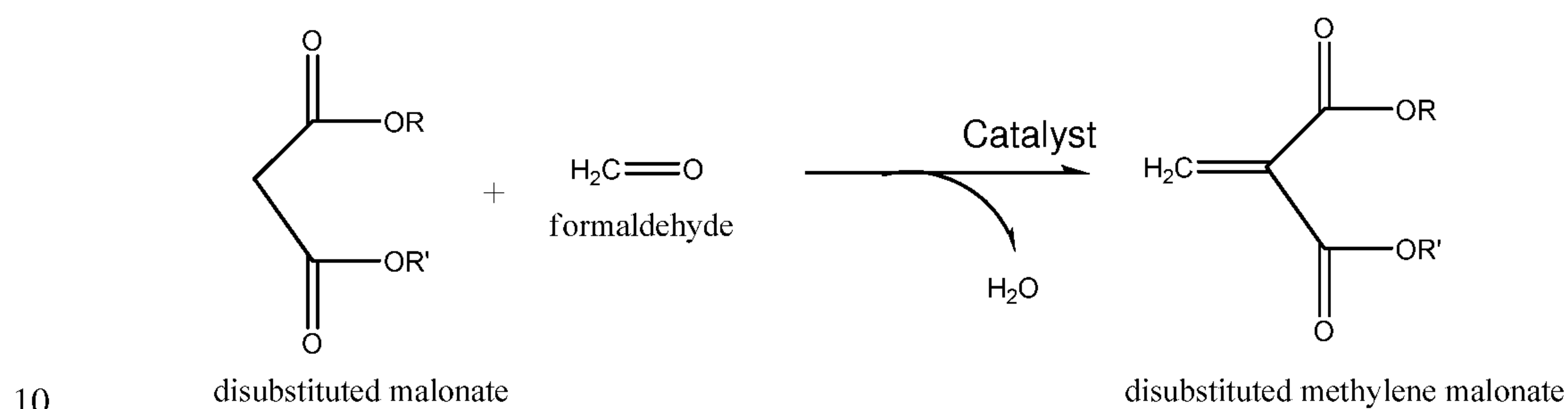
Schematic 1. Knoevenagel reaction with formaldehyde for the synthesis of a methylene malonate.
