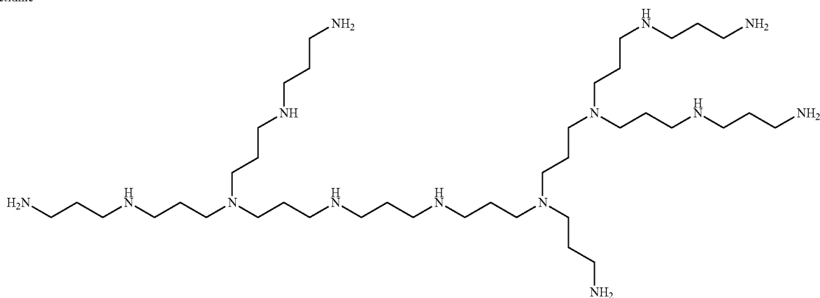
Polyazetidine
