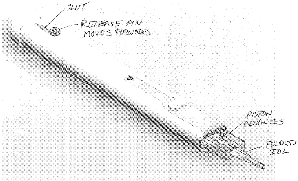
Fig. 11 - CLASP REMOVED
