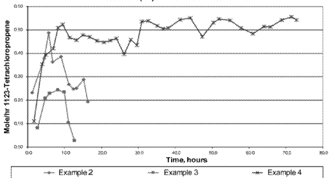
Figure 5: Results of Examples 2-4.
