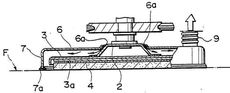
FIG. 7 PRIOR ART
