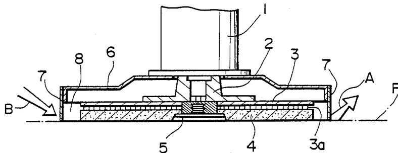
FIG. 6 PRIOR ART
