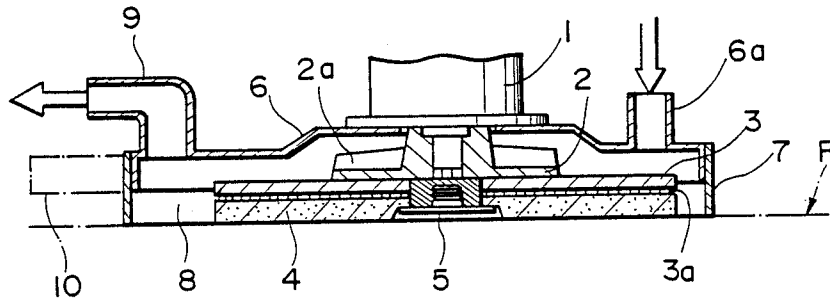
FIG. 8 PRIOR ART
