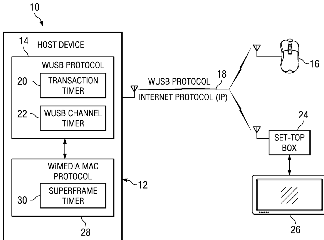
FIG. 1 (PRIOR ART)
