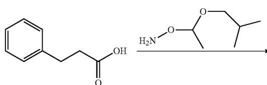
Scheme 9
