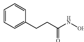
Scheme 9
