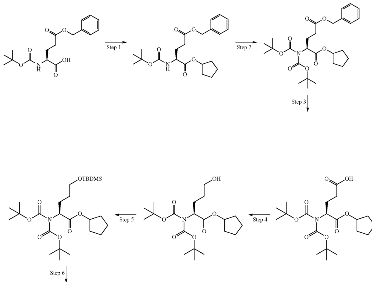
Scheme 7
