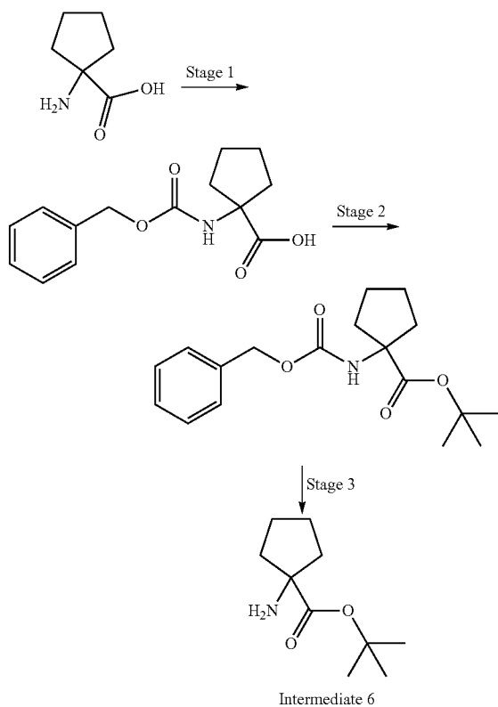
Scheme 5
