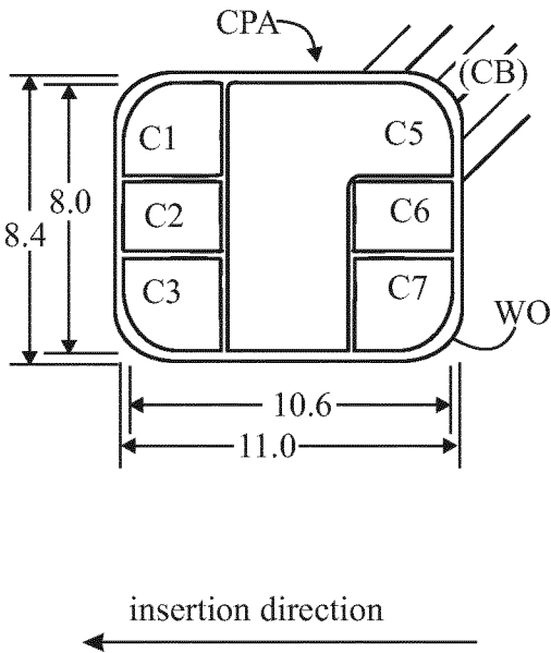
6-pad contact pattern
