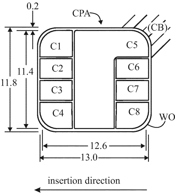
8-pad contact pattern
