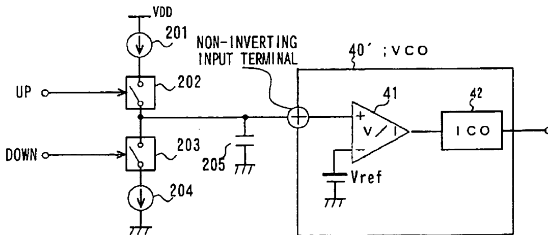
FIG. 11 PRIOR ART
