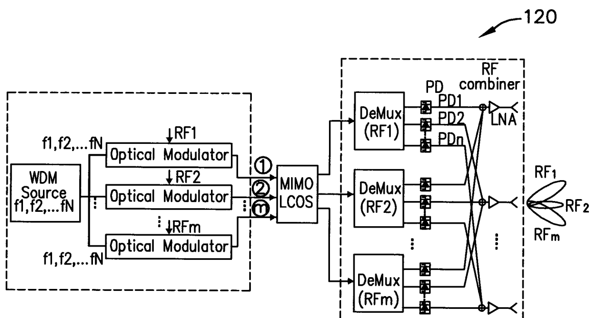
FIGURE 12 Wavelength reuse structure 2
