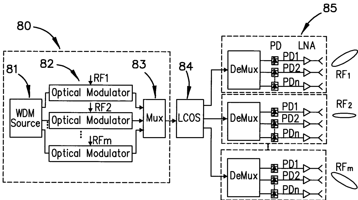
FIGURE 8 Multi-beam structure 1
