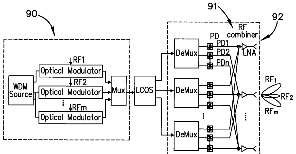
FIGURE 9 Multi-beam structure 2
