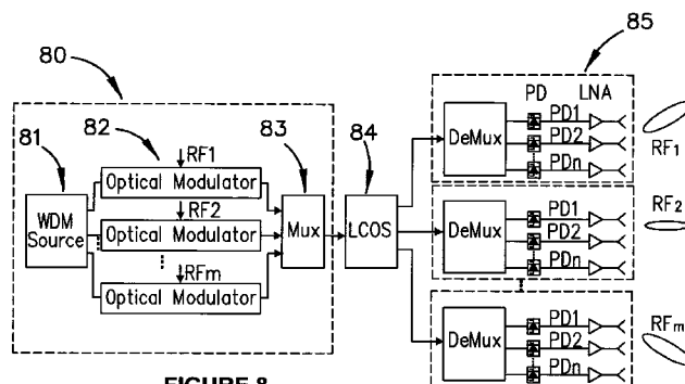
FIGURE 8 Multi-beam structure 1
