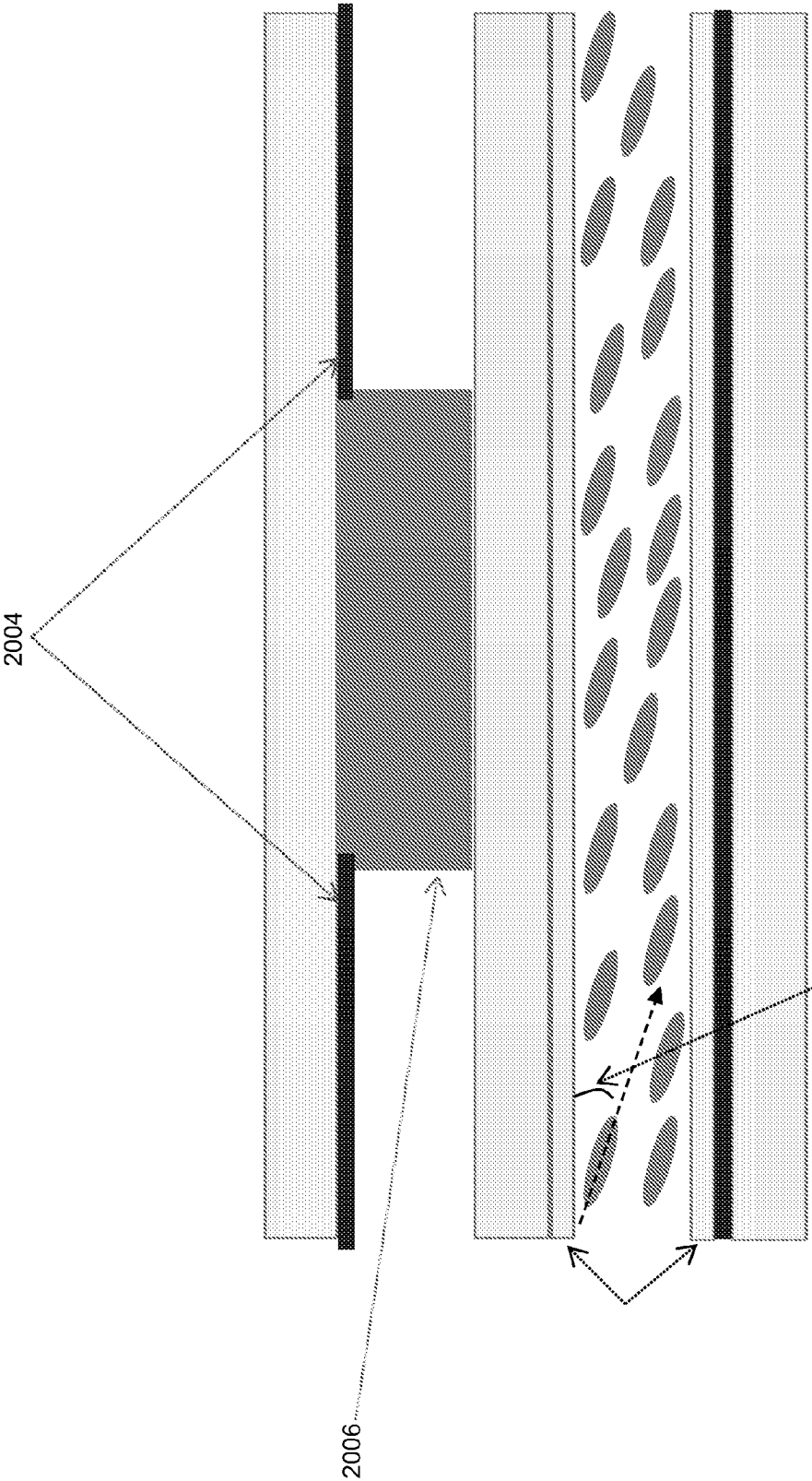
Pretilt angle FIGURE 20
