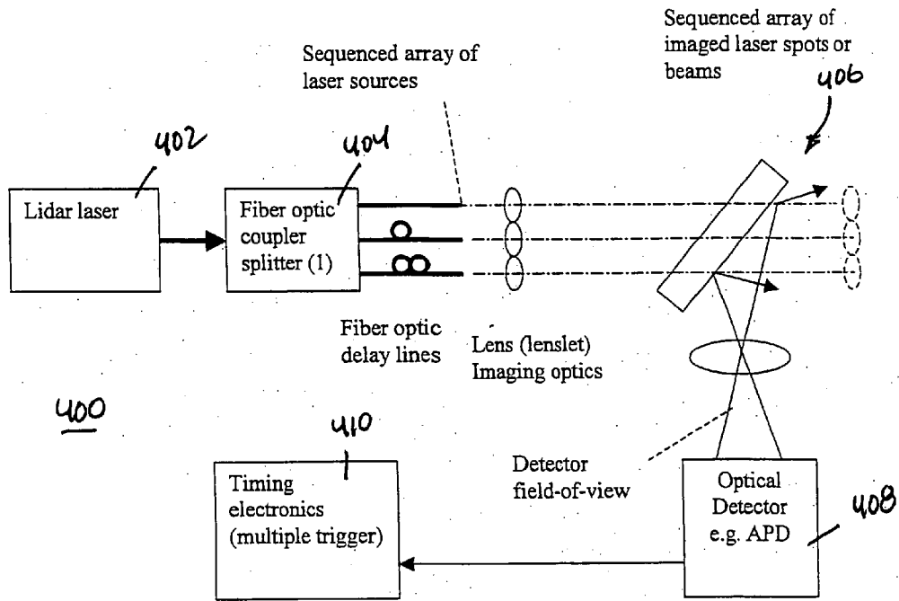
MULTIPLEXED LIDAR Version 2
