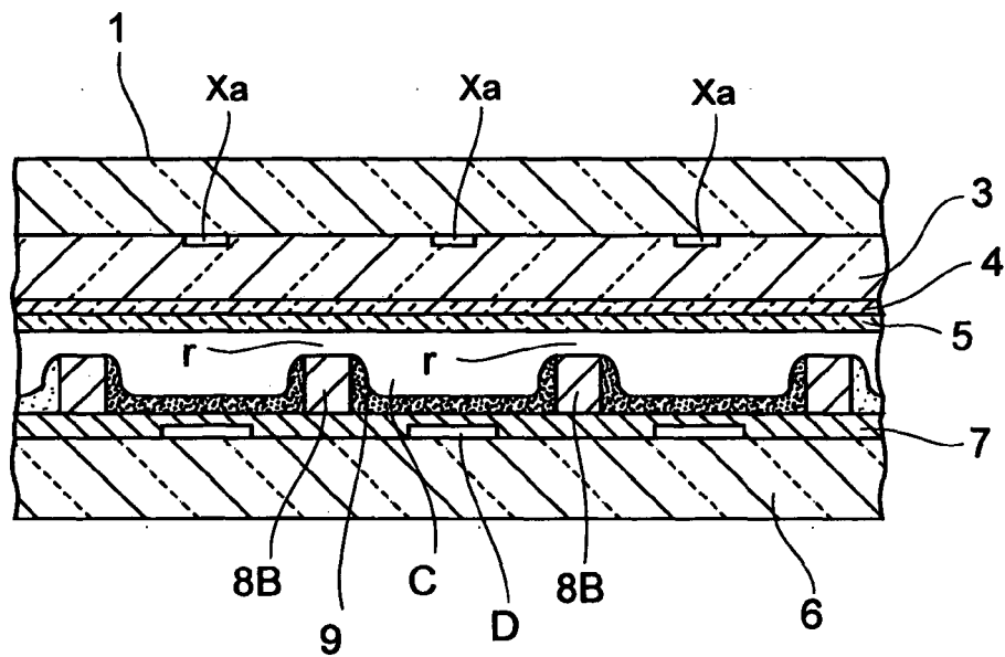
SECTION W-W
