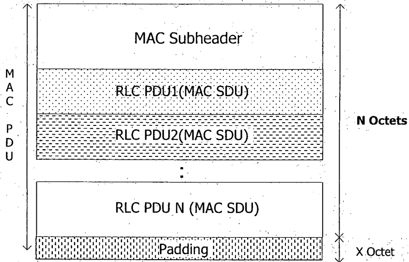
(a) MAC PDU with data and padding
