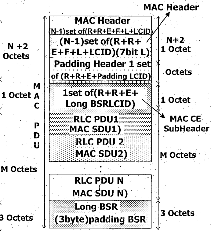
(c) case 3, explicit padding BSR
