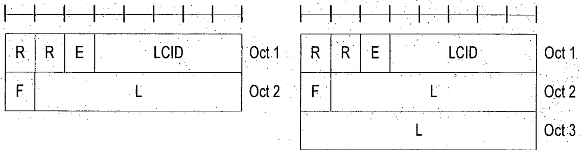
R/R/E/LCID/F/L sub-header with 7-bits L field
