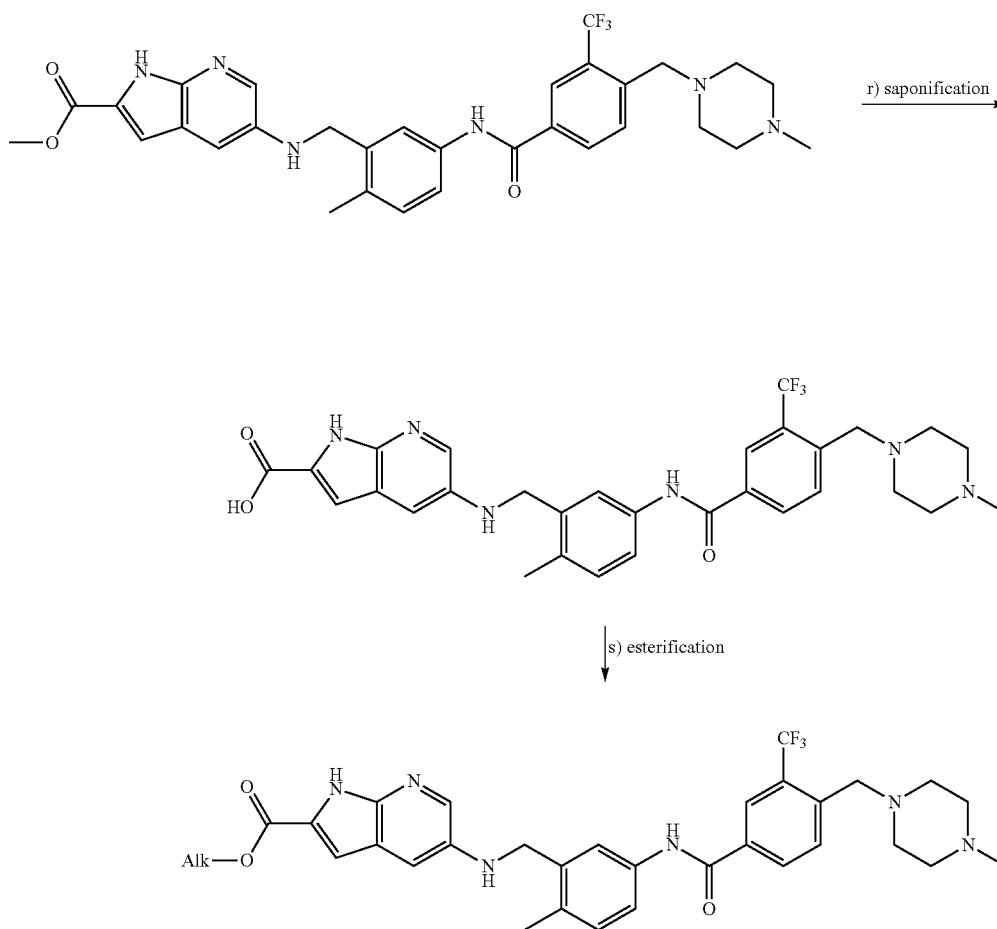
Scheme 11
