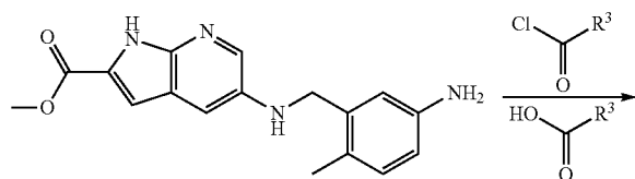
Scheme 16 - General synthesis of example C
