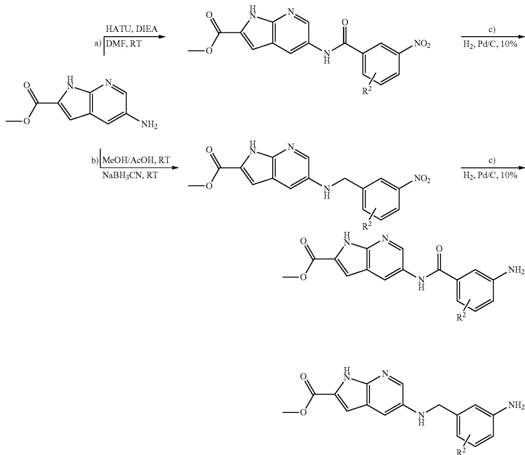
Scheme 2
