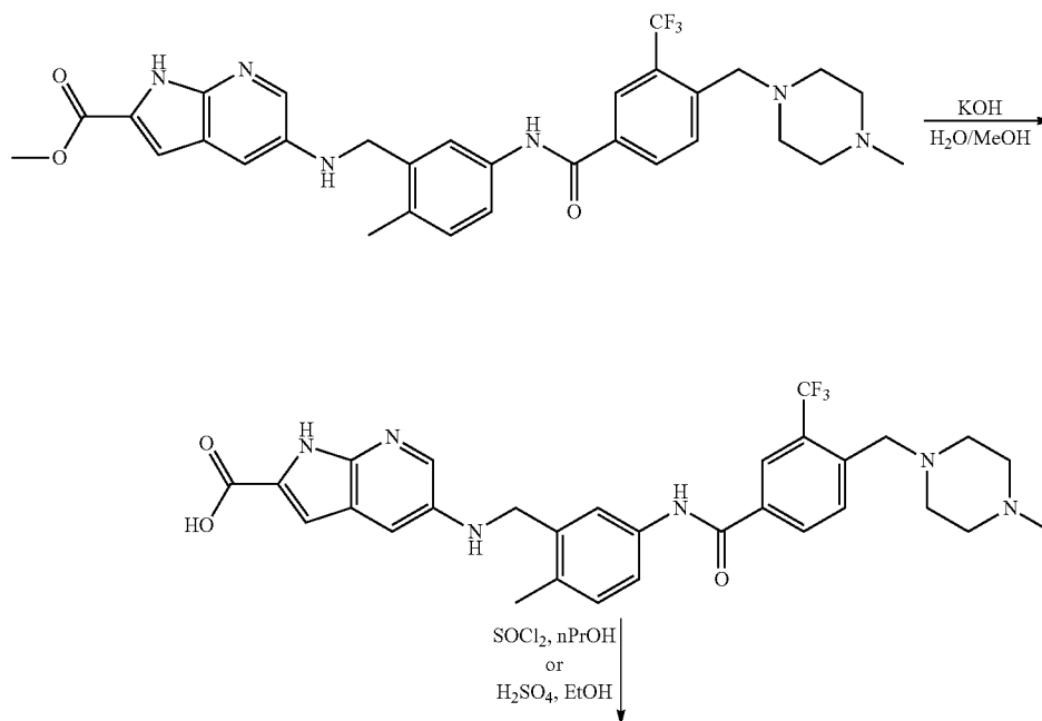
Scheme 24 - General synthesis scheme of example G
