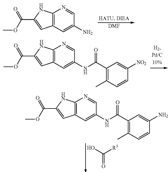
Scheme 22 - General synthesis scheme of example E
