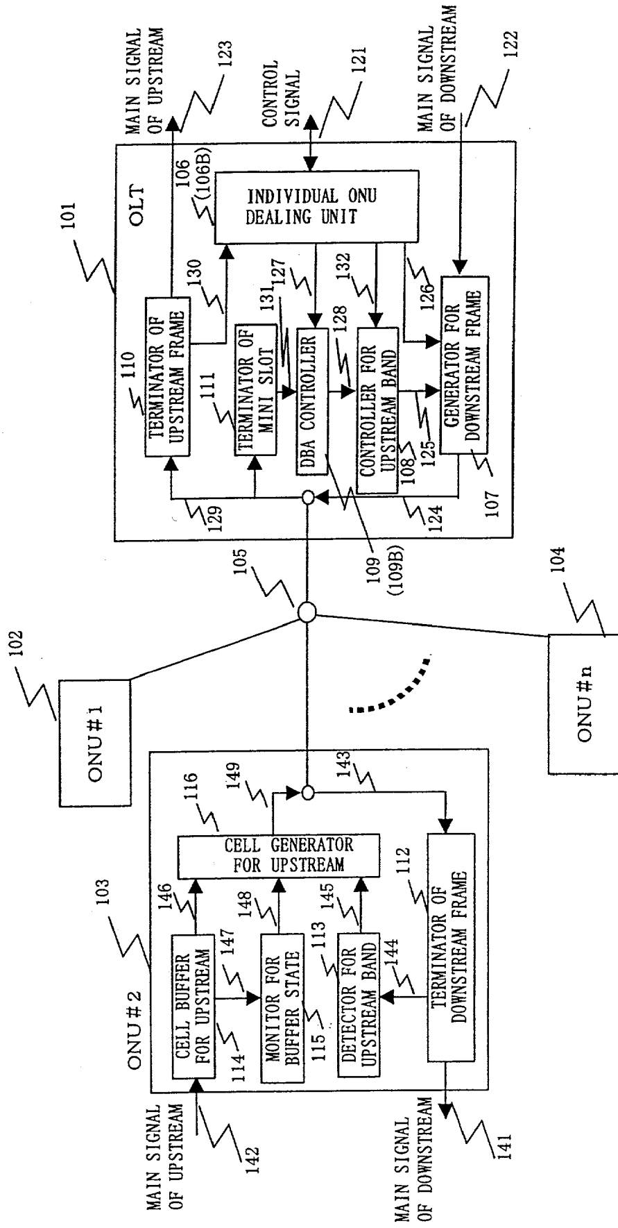
Fig. 3 RELATED ART
