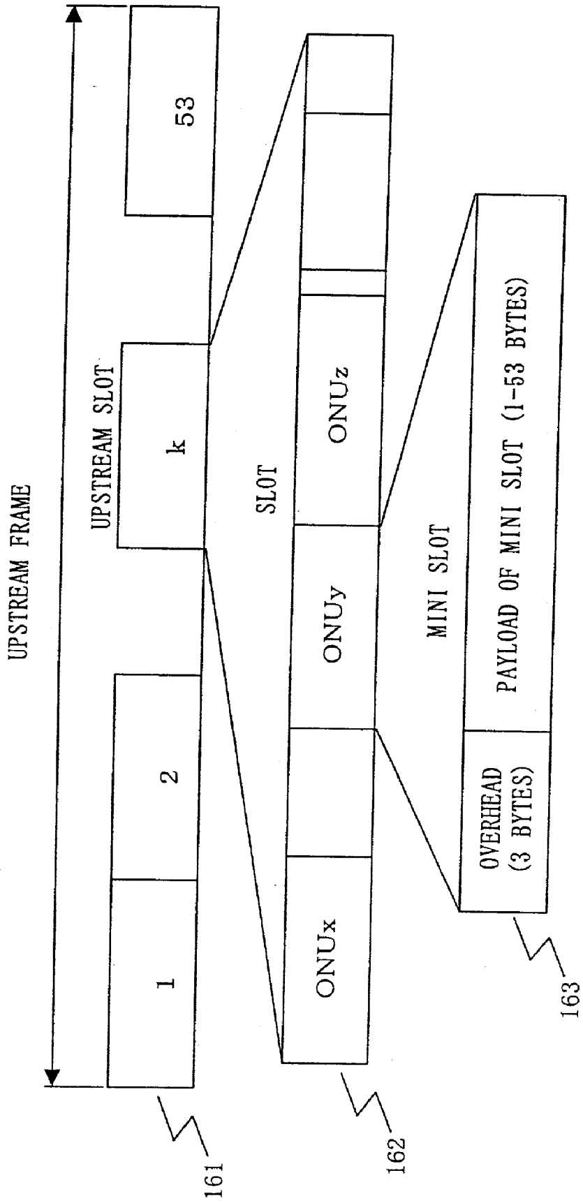
Fig. 7 RELATED ART
